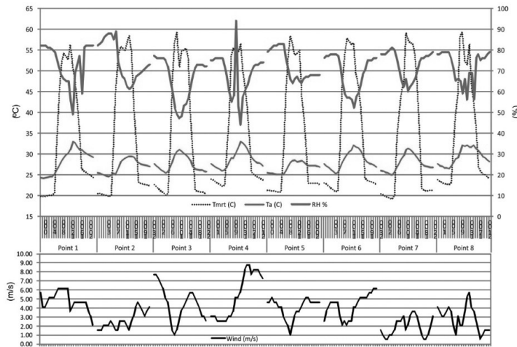
Figure 9. Graphic of Tmrt, Ta, RH and Wind speed measurement data obtained from 8 points on 10 October.
