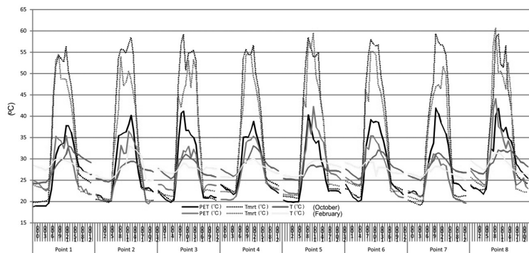
Figure 10. PET result on February and October.
