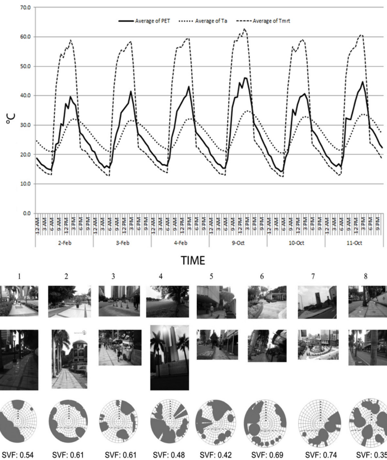
Figure 7. Environmental Characteristic at each points measurement.
