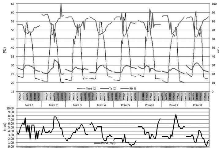
Figure 8. Graphic of Tmrt, Ta, RH and Wind speed measurement data obtained from 8 points on 2 February.
