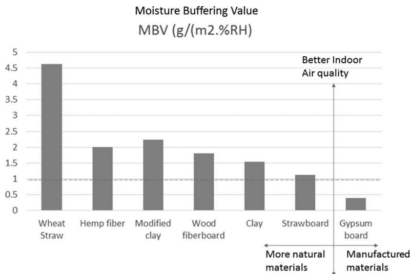
Figure 4. Comparison of MBV of natural materials that offer much better indoor air quality than typical manufactured material, leading to better human's health impact.
