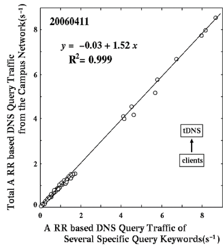
Fig.4: Total A resource record (RR) based traffic including only the specific keywords versus the PC clients based DNS query traffic including only the specific keywords through April 10th to 11th, 2006. (s -1 unit).
