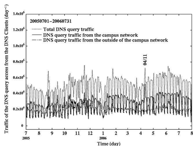
Fig.1: Total traffic of the DNS query packets to the top domain DNS server (tDNS) and the traffic from the inside- and the outside-DNS clients in a university through July 1st, 2005 to July 31st, 2006 (day-1 unit).
