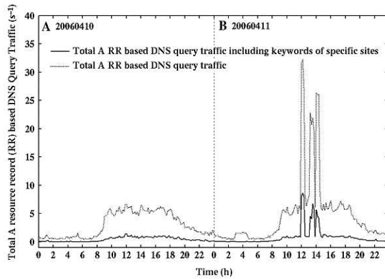
Fig.3: Total A resource record (RR) based traffic from the campus network to the top domain DNS (tDNS) server and the traffic including query keywords as specific sites through April 10th to 11th, 2006 (s -1 unit).
