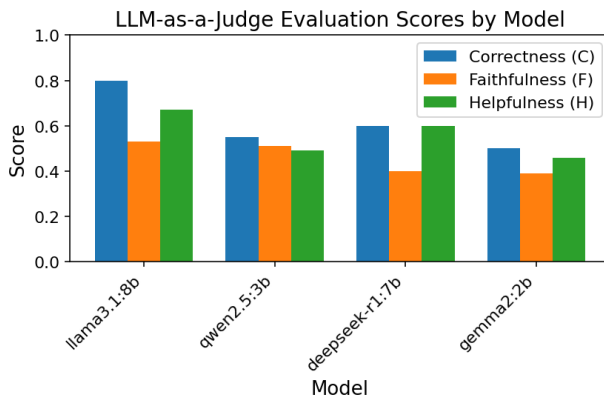
Fig. 6: LLM as Judge: Evaluation Scores by Model
