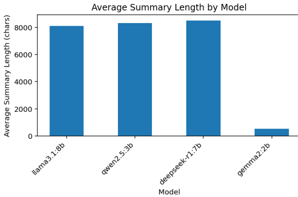
Fig. 5: Average Length of Model Summaries
