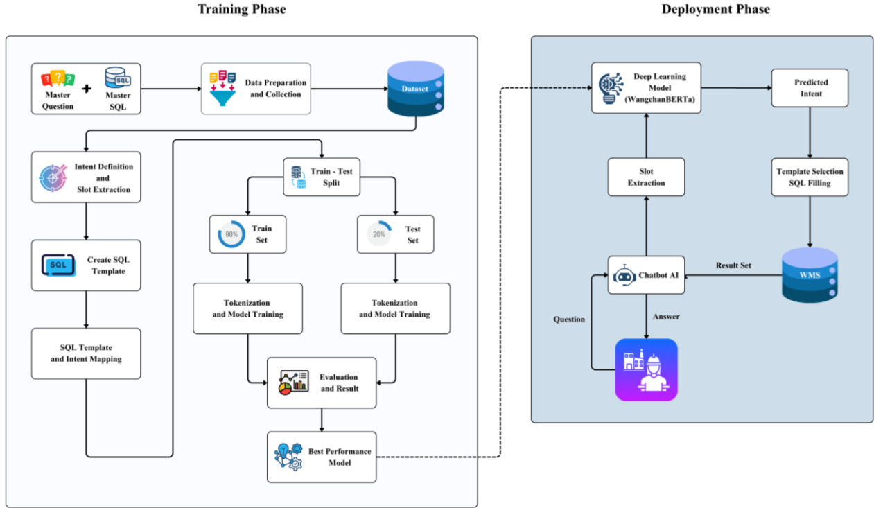
Fig. 1: Overview of the model-training and model-deployment workflow of the proposed Thai NL2SQL chatbot system
