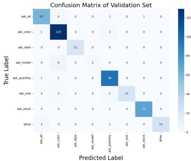
Fig. 2: Confusion matrix showing the number of predictions made for each intent class
