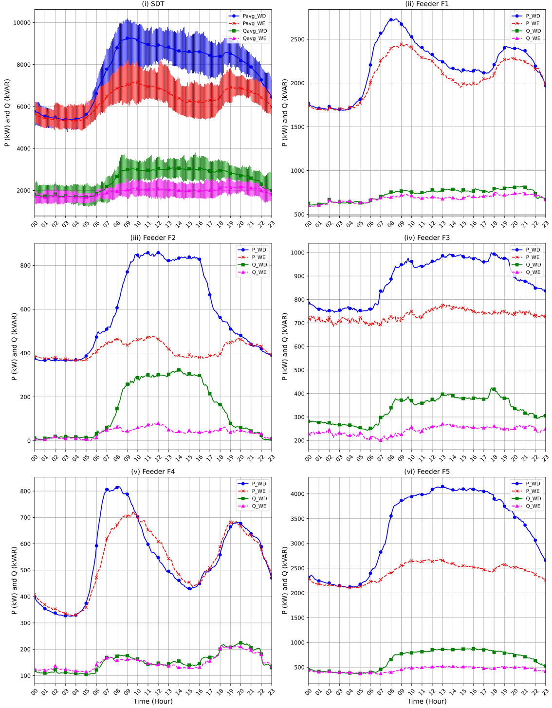
Fig. 1: Average daily load profiles: (i) Substation distribution transformer (ii) F1-Commerical feeder (iii) F2-Industrial feeder (iv) F3-Industrial feeder (v) F4-Mixed-type feeder (vi) F5- Mixed-type feeder.
