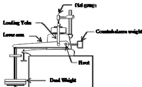
Fig. 1 one-dimensional Oedometer developed by Terzaghi
