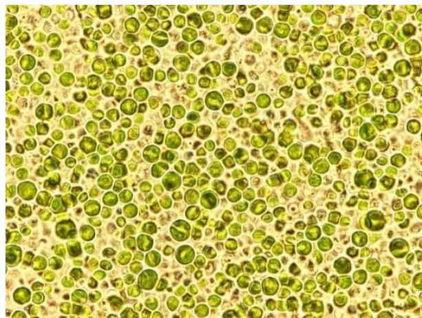
Fig. 1 Identified Nannochloropsis sp. microalgae strain
