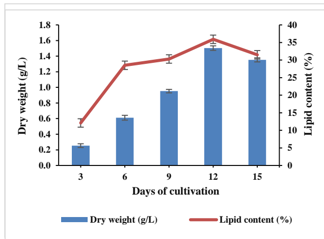
Fig. 3 Dry cell weight (g/L) and content of Nannochloropsis sp. lipid (%) in 10% POME culture.
