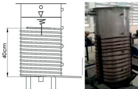
ค) S/L = 3
