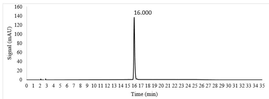
Fig. 4A. HPLC chromatogram (330 nm) of 10 µg/mL rosmarinic acid standard.
