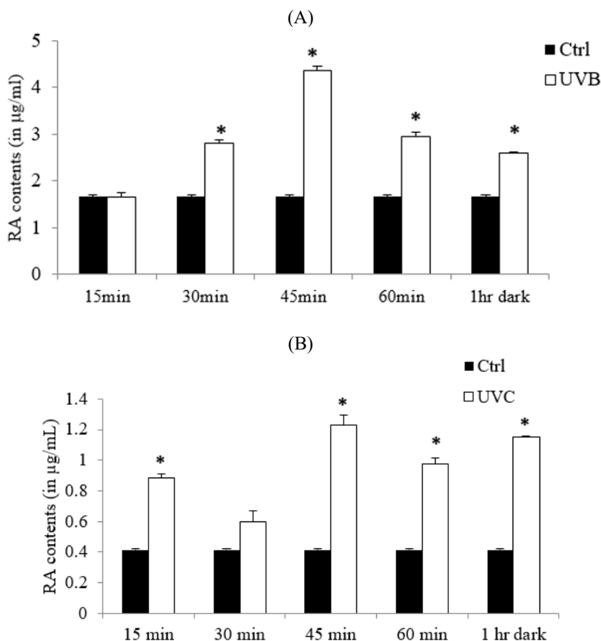
Fig. 5. Rosmarinic acid production in response to UVB (A) and UVC (B) treatments. The data represent the average of three independent biological replicates and comparison with control. The vertical bars indicate the standard errors. The statistical analysis of differences between control and each time point of treatment were performed by 2-tailed T test, p < 0.05 is indicated with asterisk (*).
