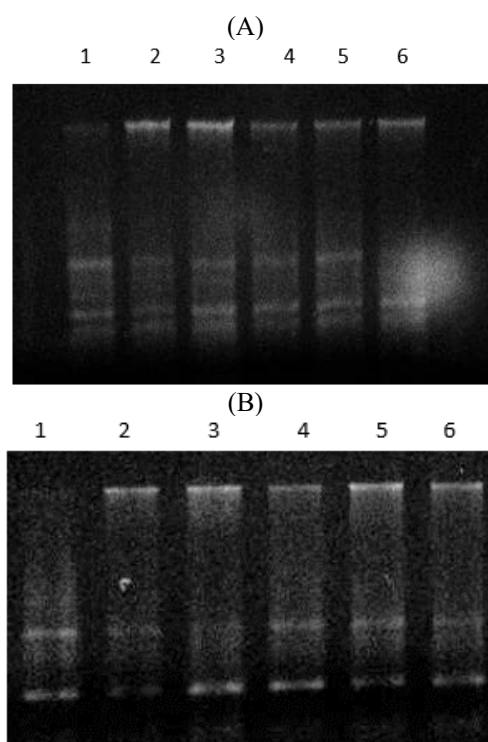
Fig. 1. Agarose gel electrophoresis of isolated total RNA from O. aristatus at different time points after UVB (A), and UVC (B) treatments. Lane 1 at 0 min as control, lane 2 at 15 mins, lane 3 at 30 mins, lane 4 at 45 mins, lane 5 at 60 mins, and lane 6 at 1 hr dark recovery.
