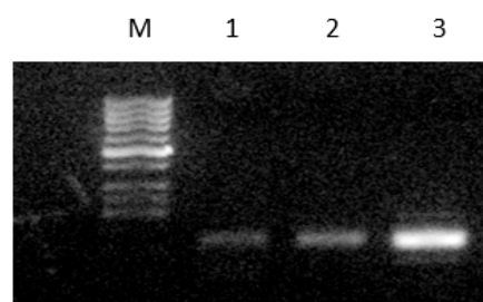
Fig. 2. Reverse transcription-polymerase chain reaction (RT-PCR) analysis of O. aristatus genes. Lane 1 represents the PCR product for the hpr gene (~250 bp), Lane 2 is the PCR product for 18S rRNA (265 bp), and Lane 3 is the PCR product for matK (235 bp).
