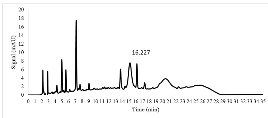
Fig. 4B. HPLC chromatogram (at wavelength 330 nm) of rosmarinic acid identified in O. aristatus leaves before UVB treatment and the concentration determined was 0.4961 µg/mL.
