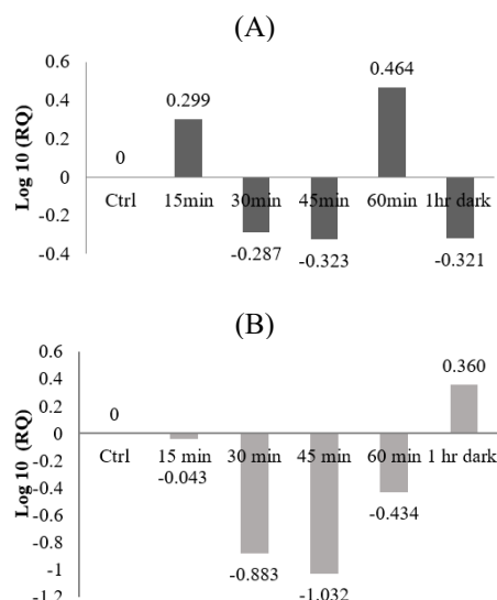
Fig. 6. The relative expression of hpr in O. aristatus after short-term UVB (A) and UVC (B) treatments. The bar graph showing the log-10 (RQ) value of hpr measured at 15 mins, 30 mins, 45 mins, 60 mins, and 1 hour dark recovery after UV treatment, and control (without UVB or UVC treatment, respectively).
