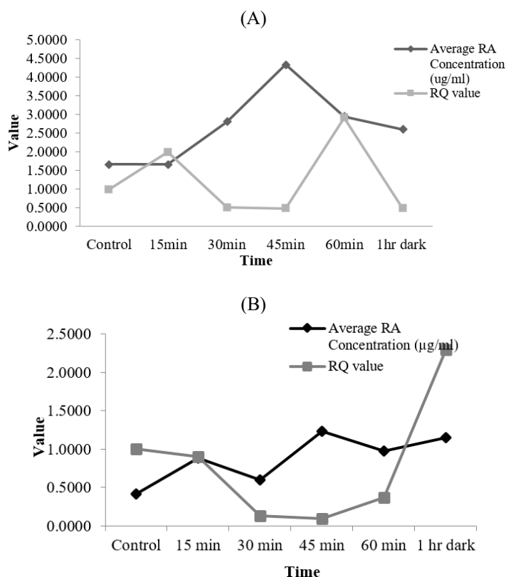
Fig. 7. Correlation between the RA production and hppr expression after UVB (A) and UVC (B) treatments. The average RA concentration denoted the average RA concentration of three dependent replicates, whereas the RQ value denoted the relative expression value of hppr gene after UVB or UVC treatments, respectively.
