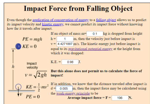
Fig. 23. impact force from falling object calculator, EVA 10 mm.
