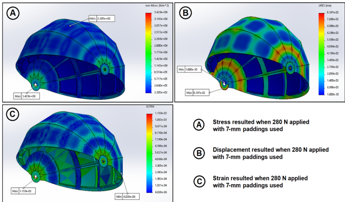
Fig. 22. FEA Simulation for model with 7-mm EVA paddings.
