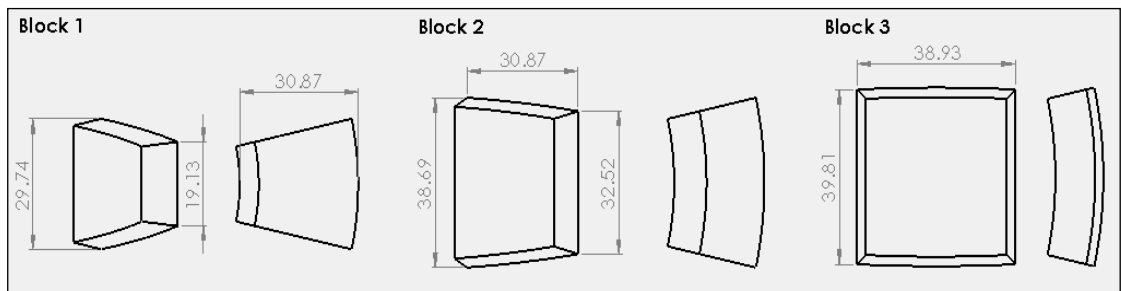
Fig. 12. Dimensions of paddings.
