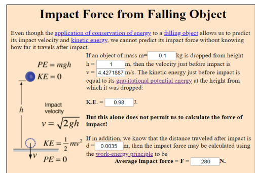
Fig. 21. impact force from falling object calculator, EVA 7-mm. thickness.
