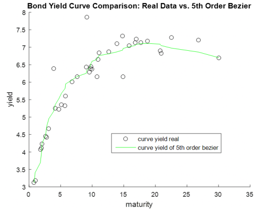
Fig. 3. Comparison of bond yield curves: real data vs. 5th order bezier for bonds data on 27 July 2023.
