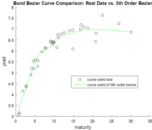
Fig. 5. Comparison of bond yield curves: real data vs. 5th order bezier for bonds data on 28 July 2023.
