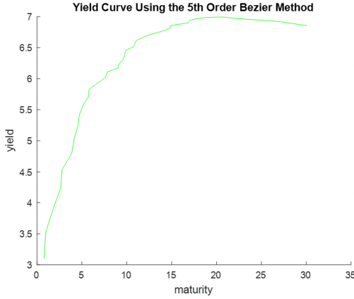
Fig. 4. Bond yield curve using the 5th order bezier method for bond data on 28 July 2023.
