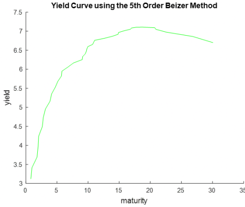
Fig. 2. Bond yield curve using the 5th order bezier method for bond data on 27 July 2023.
