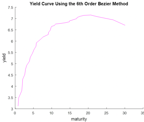
Fig. 6. Bond yield curve using the 6th order bezier method for bond data on 27 July 2023.
