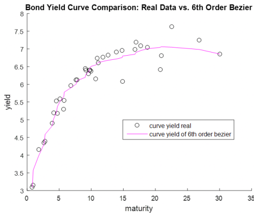
Fig. 9. Comparison of bond yield curves: real data vs. 6th order bezier for bonds data on 28 July 2023.
