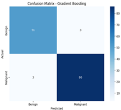
Fig. 20. CM of Gradient Boost ensemble.
