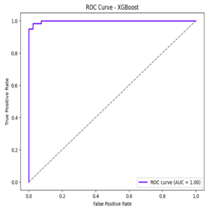
Fig. 15. ROC of XGBoost.
