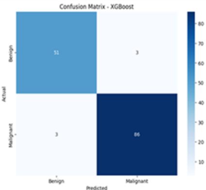
Fig. 21. CM of XGBoost ensemble.
