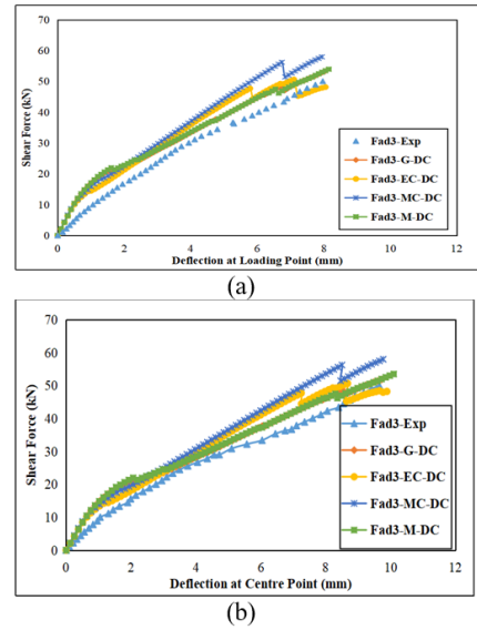
Fig. 14. Shear Force (kN) vs Deflection (mm) for Fad3 beam (a) at Loading Point (b) at Centre Point.
