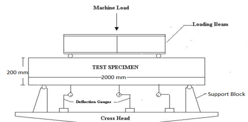
Fig. 3. Experimental setup.
