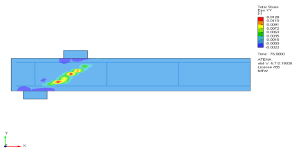
Fig. 15. Strains obtained using Numerical Analysis for Dad1 beam.
