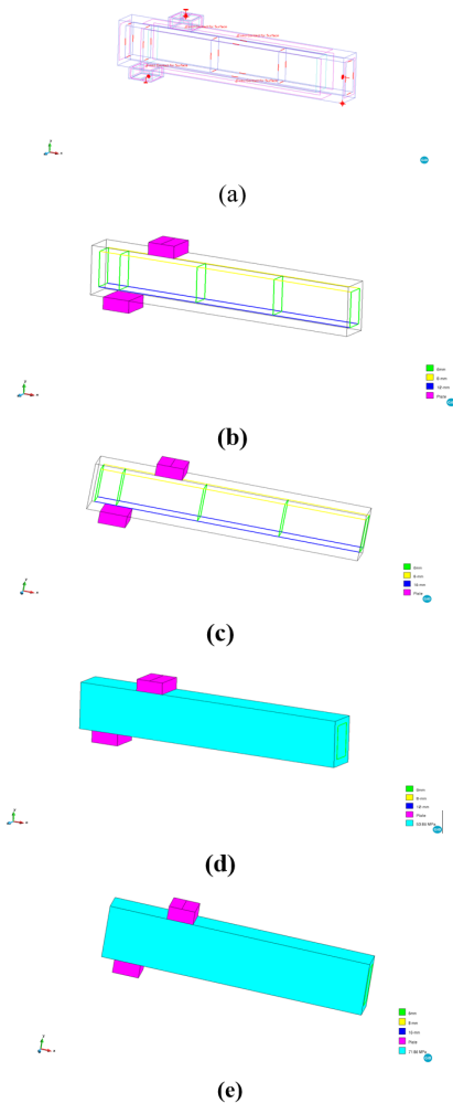
Fig. 4. Beam modelling in ATENA (a) Beam with constraints and monitor points (b) & (c) Beam showing the assigned material for reinforcement for Dad1 beam and Fad1 beam respectively (d) & (e) Dad1 & Fad1 beams assigned with concrete respectively.
