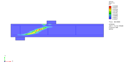
Fig. 19. Strains obtained using Numerical Analysis for Fad2 beam.
