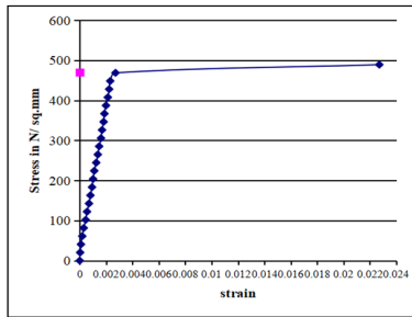
Fig. 24. Strains obtained using Numerical Analysis for Fad3 beam.
