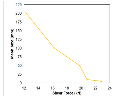
Fig. 25. Mesh size (mm) vs Shear Force (kN) for a PCC beam of strength 50 MPa.
