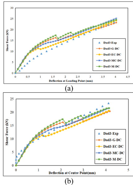
Fig. 11. Shear Force (kN) vs Deflection (mm) for Dad3 beam (a) at Loading Point (b) at Centre Point.
