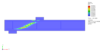
Fig. 16. Strains obtained using Numerical Analysis for Dad2 beam.
