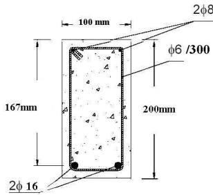
Fig. 2. Cross-section details for specimens Fad1, Fad2, and Fad3.
