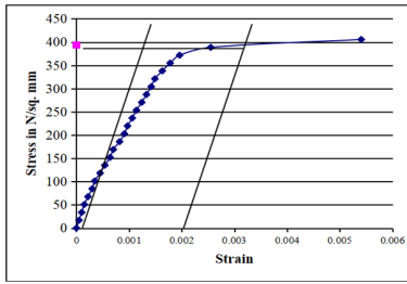
Fig. 23. Stress-Strain curve of 12mm diameter steel bar.
