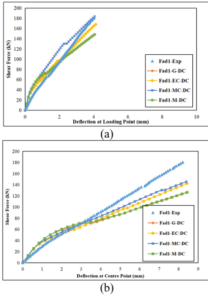
Fig. 12. Shear Force (kN) vs Deflection (mm) for Fad1 beam (a) at Loading Point (b) at Centre Point.
