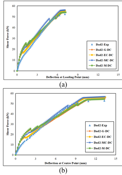
Fig. 10. Shear Force (kN) vs Deflection (mm) for Dad2 beam (a) at Loading Point (b) at Centre.
