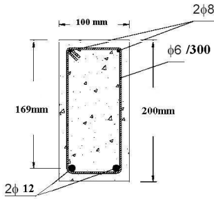
Fig. 1. Cross-section details for specimens Dad1, Dad2 and Dad3.
