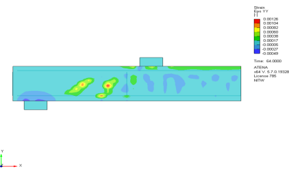
Fig. 17. Strains obtained using Numerical Analysis for Dad3 beam.
