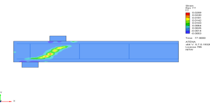
Fig. 18. Strains obtained using Numerical Analysis for Fad1 beam.
