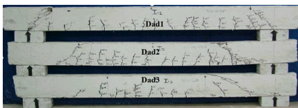
Fig. 7. Photographs of tested beams for Series-D.
