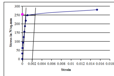
Fig. 21. Stress-Strain curve of 6mm diameter steel bar.
