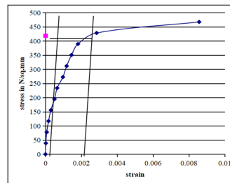
Fig. 22. Stress-Strain curve of 6mm diameter steel bar.
