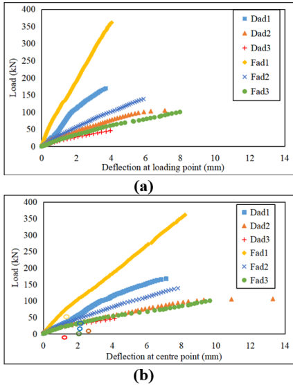
Fig. 6. (a) Load vs Deflection at loading point for Series-D and Series-F (b) Load vs Deflection at centre point for Series-D and Series-F, “O” indicates cracking load points.
