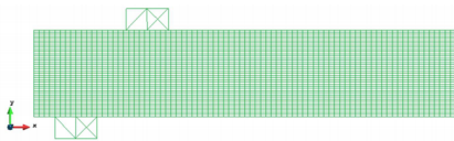
Fig. 5. Beam with mesh size of 5 mm.
