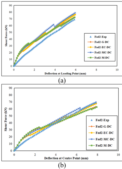
Fig. 13. Shear Force (kN) vs Deflection (mm) for Fad2 beam (a) at Loading Point (b) at Centre Point.
