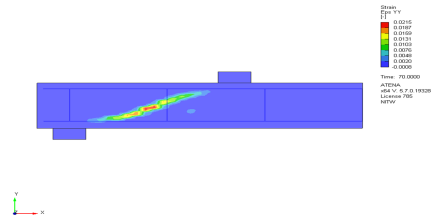
Fig. 20. Strains obtained using Numerical Analysis for Fad3 beam.
