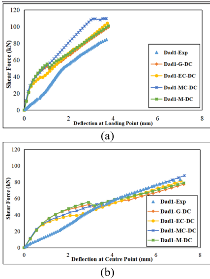
Fig. 9. Shear Force (kN) vs Deflection (mm) for Dad1 beam (a) at Loading Point (b) at Centre Point.
