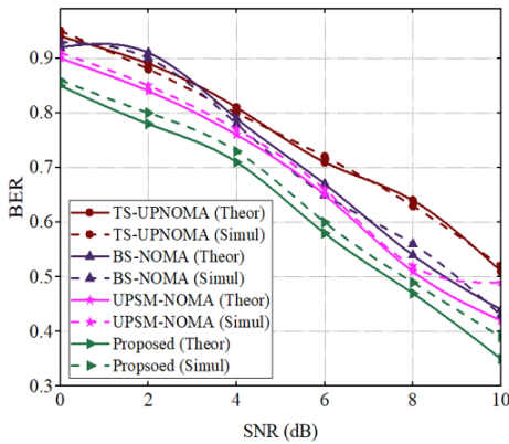
Fig. 5. BER comparison.
