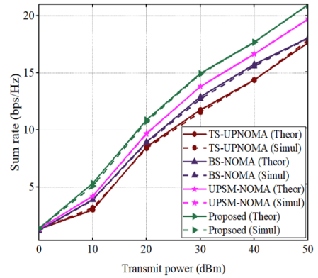
Fig. 6. Comparison of sum rate.
