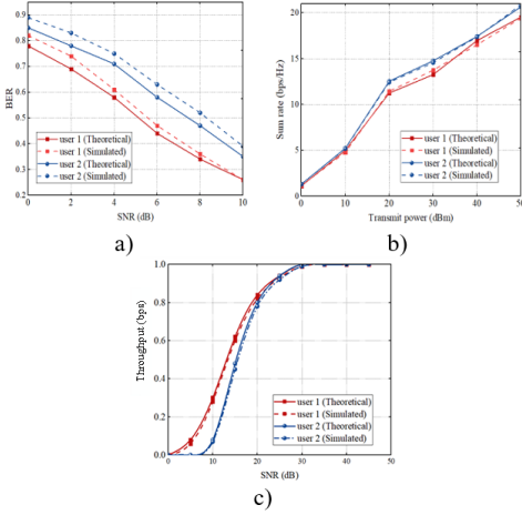
Fig. 4. Performance of proposed: a) BER, b) sum rate, c) throughput.
