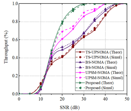
Fig. 7. Throughput comparison.
