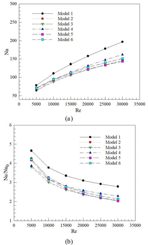
Fig. 10. The variations of (a) Nu and (b) Nu/Nu_0 various Re .
