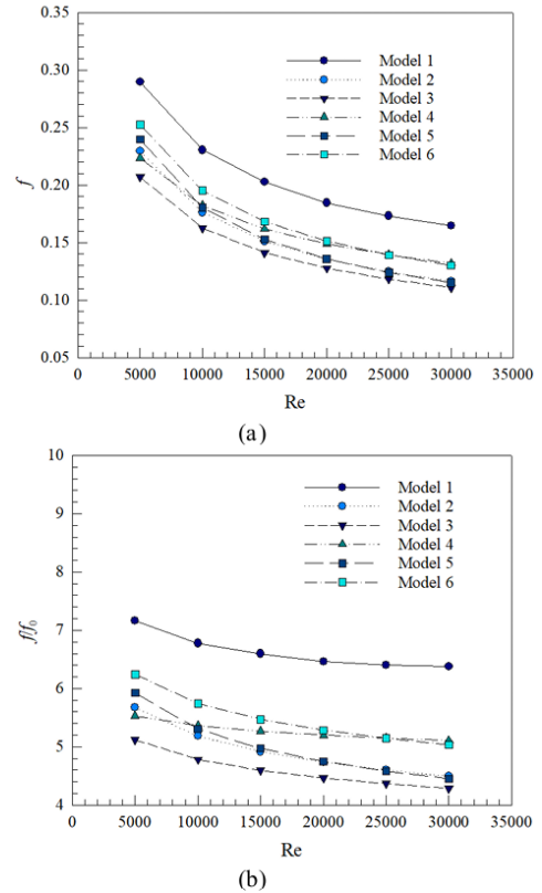
Fig. 11. Variations of (a) f and (b) f/f_0 versus Re .
