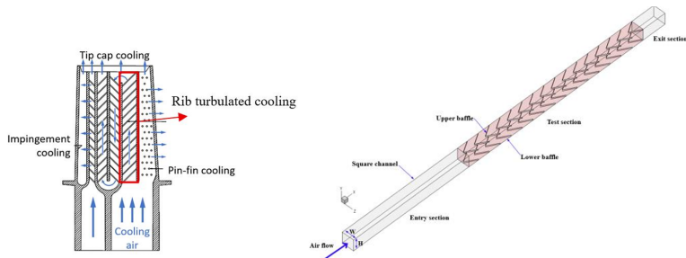
Fig. 1. (a) Illustration showing internal cooling methods used in modern gas turbine blades, and (b) a close-up view of the cooling passage.
