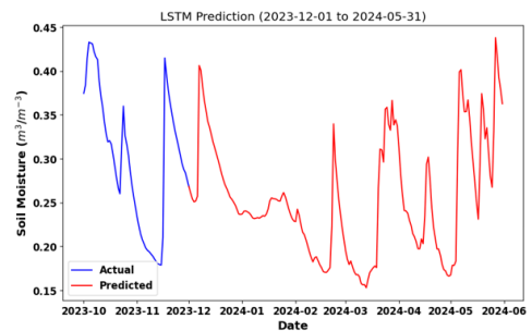
Fig. 12. Predicted soil moisture result from December 1, 2023 to May 31, 2024.
