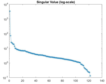
Fig. 2. Singular values of Hankel matrix for the BDMS stock prices.
