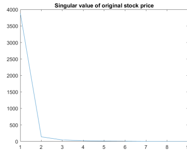
Fig. 4. Singular values of Hankel matrix for the BDMS stock prices.
