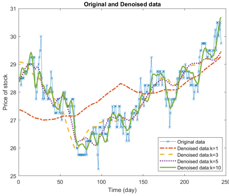
Fig. 1. BDMS stock price and its denoised data using HSVD approach with k = 1, 3, 5, 10 .
