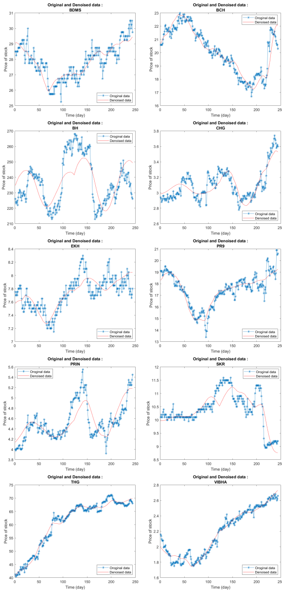
Fig. 3. The actual stock prices (in blue color) of the 10 companies from healthcare sector in Thailand and the corresponding trend (in red color) from the HSVD approach with k = 5 .
