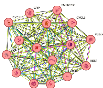
Fig. 3 String DB protein-protein interaction.
