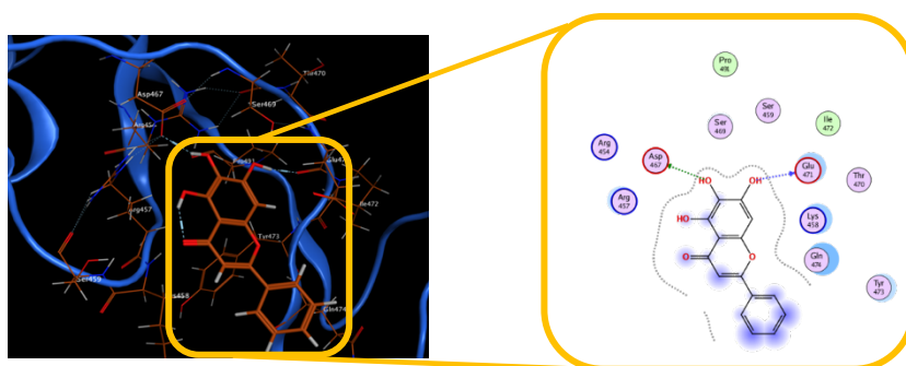
Fig. 4 Molecular interaction diagram of baicalein in the ACE2 binding site. In the interaction analysis, hydrophobic contacts and van der Waals interactions were treated as distinct interaction types. Hydrophobic contacts refer to contacts involving nonpolar regions of the ligand and protein residues, whereas van der Waals interactions represent short-range nonbonded contacts. These interaction types were therefore described in the text rather than distinguished by additional graphical modifications to the Fig. 4.
