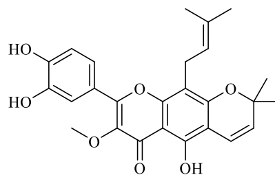
8-(3,4-dihydroxyphenyl)-5-hydroxy-7-methoxy-2,2-dimethyl-10-(3-methylbut-2-en-1-yl)2H,6H-pyrano[3,2-g]chromen-6-one
