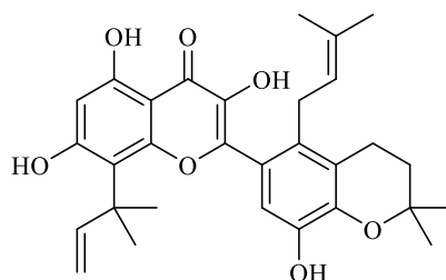
3,5,7-trihydroxy-2-(8-hydroxy-2,2-dimethyl-5-(3-methylbut-2-en-1-yl)chroman-6-yl)-8-(2-methylbut-3-en-2-yl)-4H-chromen-4-one
