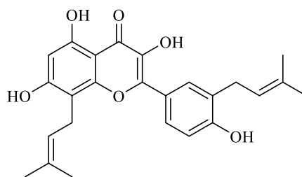
3,5,7-Trihydroxy-2-[4-hydroxy-3-(3-methyl-2-butenyl)phenyl]-8-(3-methyl-2-butenyl)-4H-1-benzopyran-4-one
