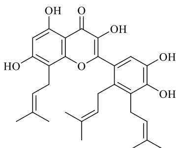
2-(4,5-dihydroxy-2-(4,5-dihydroxy-2,3-bis(3-methylbut-2-enyl)phenyl)-3,5,7-trihydroxy-8-(3-methylbut-2-enyl)chromen-4-one
