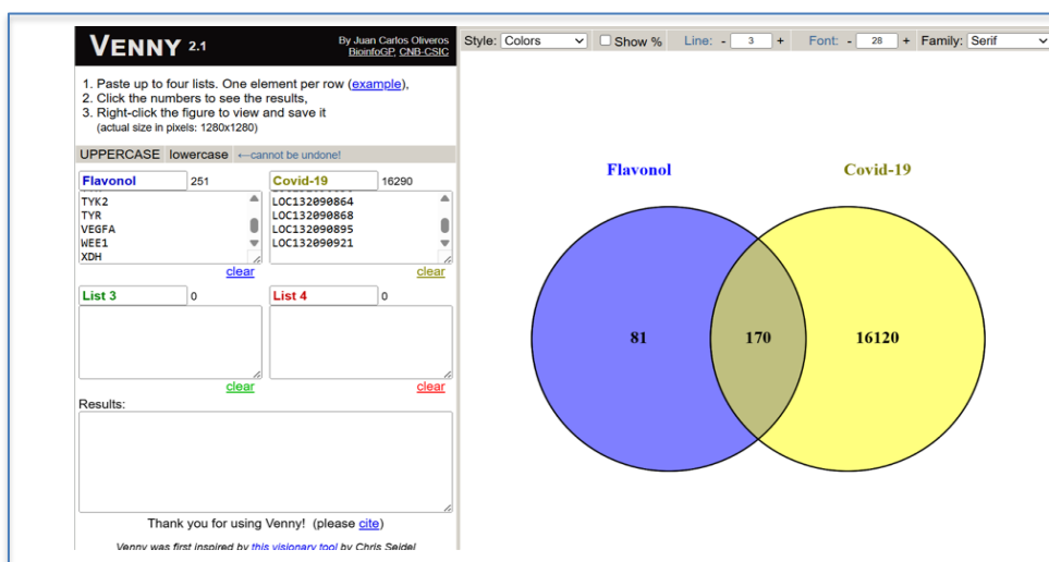
Fig. 2 Venn diagram (purple: Flavonol-associated proteins; yellow: COVID-19-associated proteins; Overlap: Indicates proteins that both interact with flavonol compounds and are involved in COVID-19 pathology).
