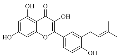
3,5,7-Trihydroxy-2-[4-hydroxy-3-(3-methyl-2-butenyl)phenyl]-4H-1-benzopyran-4-one
