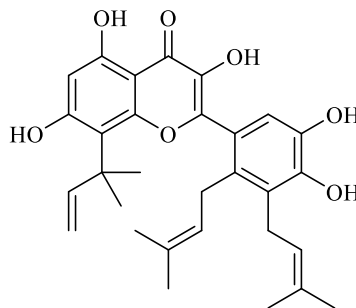
2-(4,5-Dihydroxy-2-(3-methyl-but-2-enyl)-3-((E)-3-methyl-but-2-enyl)-phenyl)-8-(1,1-dimethyl-allyl)-3,5,7-trihydroxy-1-benzopyran-4-one
