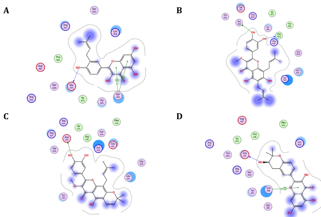
Fig. 5. Spatial arrangement of (a) Isolicoflavonol (SF6), (b) Brousoflavonol B (SF8), (c) Brousoflavonol A (SF11), and (d) Glycyrrhiza flavonol A (SF16) with protein Note: Dotted lines indicated hydrogen bonding.
