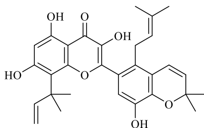
3,5,7-trihydroxy-2-[8-hydroxy-2,2-dimethyl-5-(3-methylbut-2-enyl)chromen-6-yl]-8-(2-methylbut-3-en-2-yl)chromen-4-one
