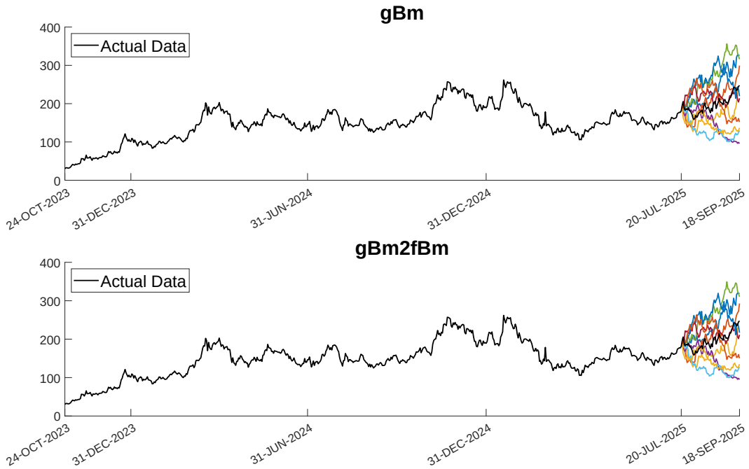
Fig. 2. Comparison of ten simulated paths with the actual observed data.
