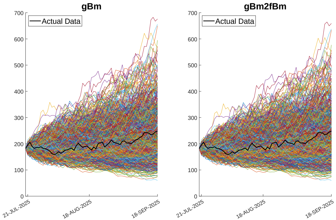
Fig. 3. Comparison of the full set of simulated trajectories (1000 paths) with the actual data.
