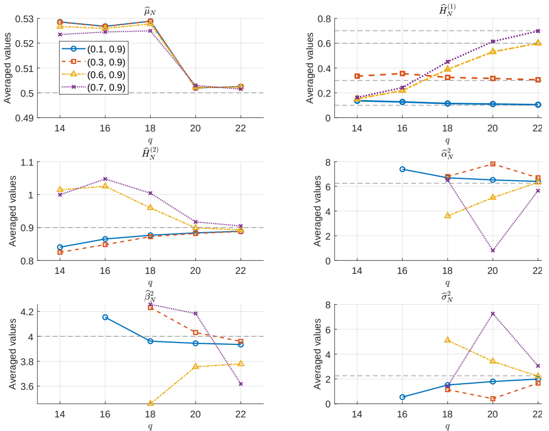
Fig. 1. Averaged values of the proposed estimators for representative Hurst parameter pairs: (0.1, 0.9), (0.3, 0.9), (0.6, 0.9), and (0.7, 0.9) as the sample size exponent q increases. The dashed horizontal lines indicate the corresponding true parameter values. The true model parameters are \mu = 0.5, \sigma = 1.5, \alpha = 2.5 , and \beta = 2 , with h = 1 .
