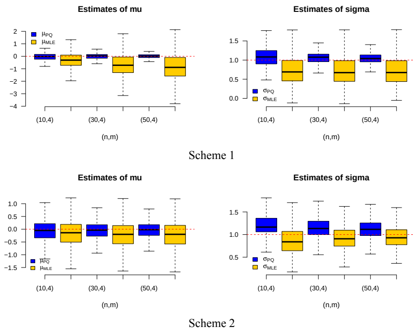
Fig. 1. Boxplots of the estimates of \mu and \sigma under Scheme 1 (top) and Scheme 2 (bottom) for \mu = 0 , \sigma = 1 , with (n, m) = (10, 4), (30, 4), (50, 4) .
