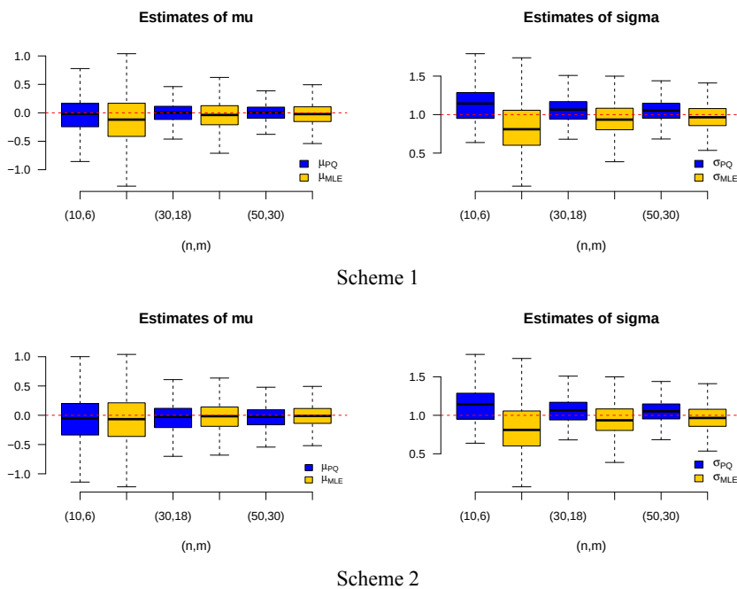
Fig. 2. Boxplots of the estimates of \mu and \sigma under Scheme 1 (top) and Scheme 2 (bottom) for \mu = 0 , \sigma = 1 , with (n, m) = (10, 6), (30, 18), (50, 30) .
