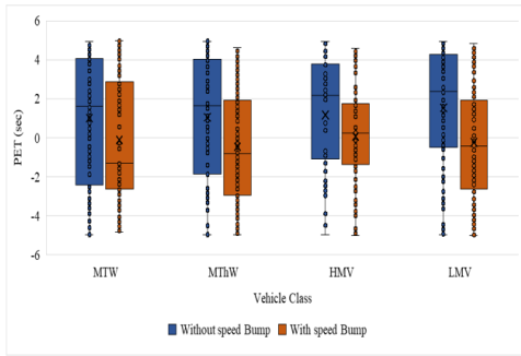
Fig. 5. Occupancy time for different vehicle categories for the scenarios without and with the speed bump.
