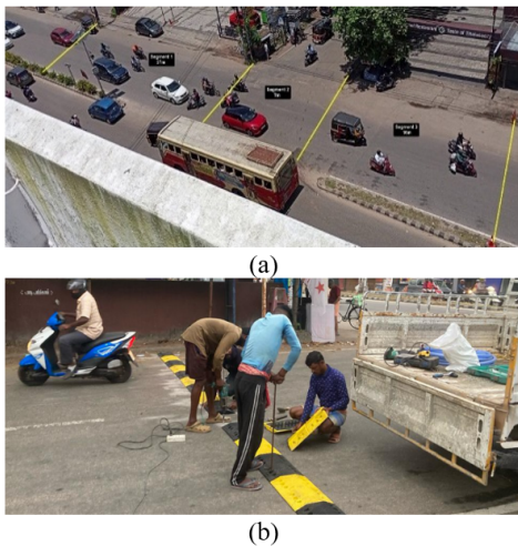
Fig. 2. Images of the study site at the CIT road intersection (a) Intersection view with segments, (b) Speed bump installation.
