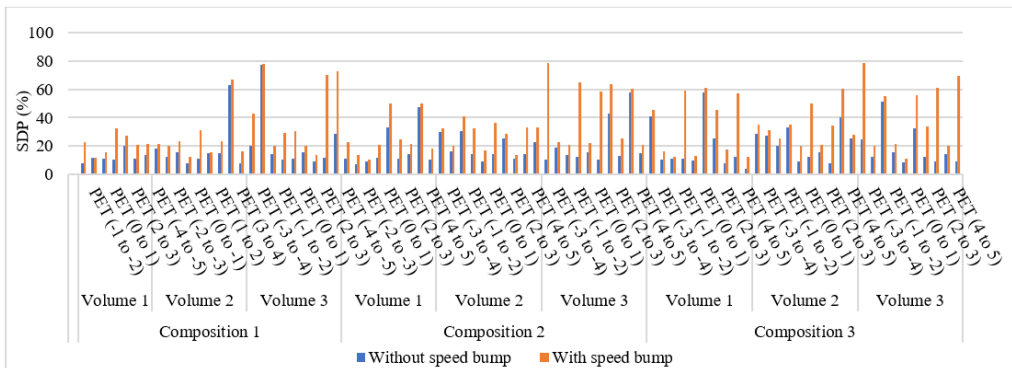
Fig. 16. Simulated SDP variation across PET ranges for the scenarios without and with the speed bump.
