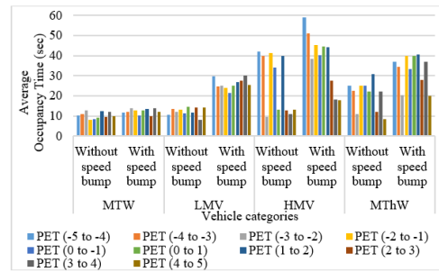
Fig. 4. Variation in occupancy time for offending vehicles across all PET ranges.
