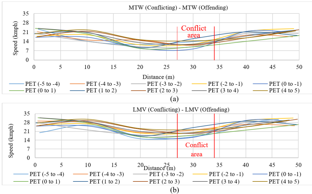
Fig. 6. Variation of speed along a major road without a speed bump when (a) MTW as the conflicting vehicle and MTW as the offending vehicle (b) LMV as the conflicting vehicle and LMV as the offending vehicle.
