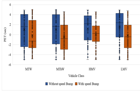
Fig. 3. Box plot of PET for different vehicle categories for the scenarios without and with the speed bump scenario.
