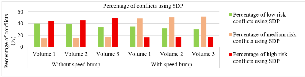
Fig. 15. Percentage conflict based on SDP across scenarios.
