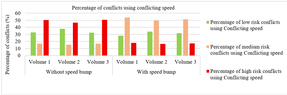
Fig. 12. Percentage conflict based on conflicting speed across scenarios.
