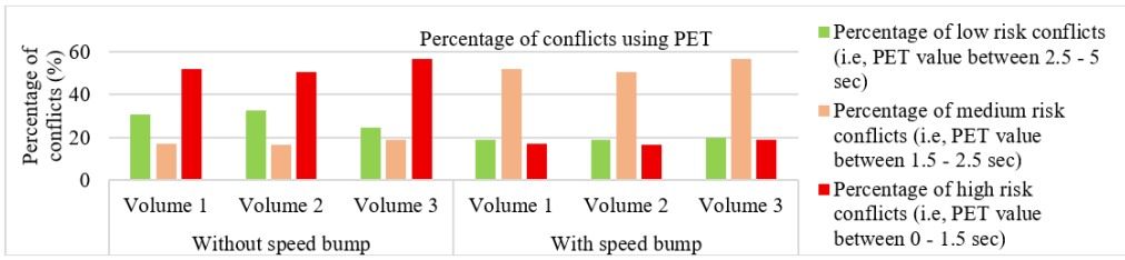
Fig. 10. Percentage Conflict based on PET across scenarios.
