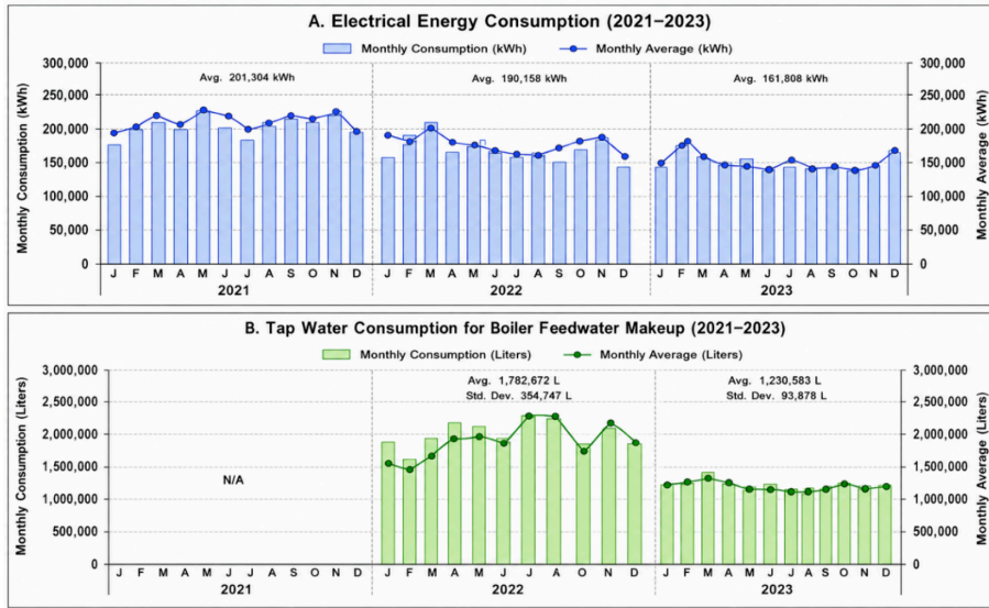
Fig. 4. Monthly electricity and water consumption during 2021–2023: (A) electricity consumption and (B) boiler feedwater makeup.
