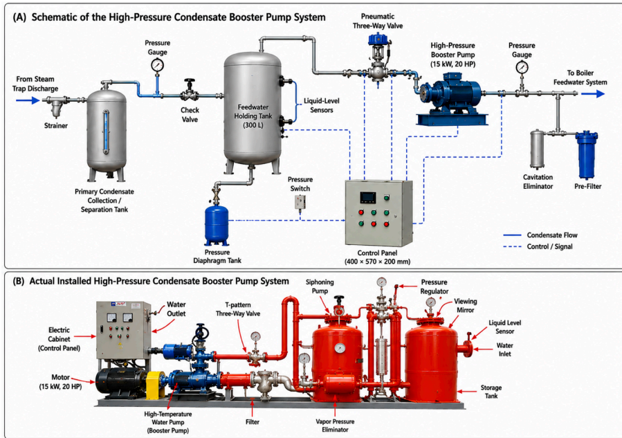
Fig. 1. High-pressure condensate return system: (A) system schematic and (B) installed system showing the booster pump, separator, storage tank, sensors, valves, and control cabinet.
