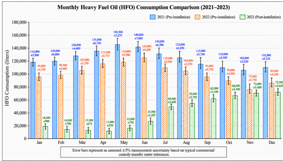
Fig. 3. Monthly HFO consumption during 2021–2023. The largest reductions occurred during January–June 2023 compared with 2022.
