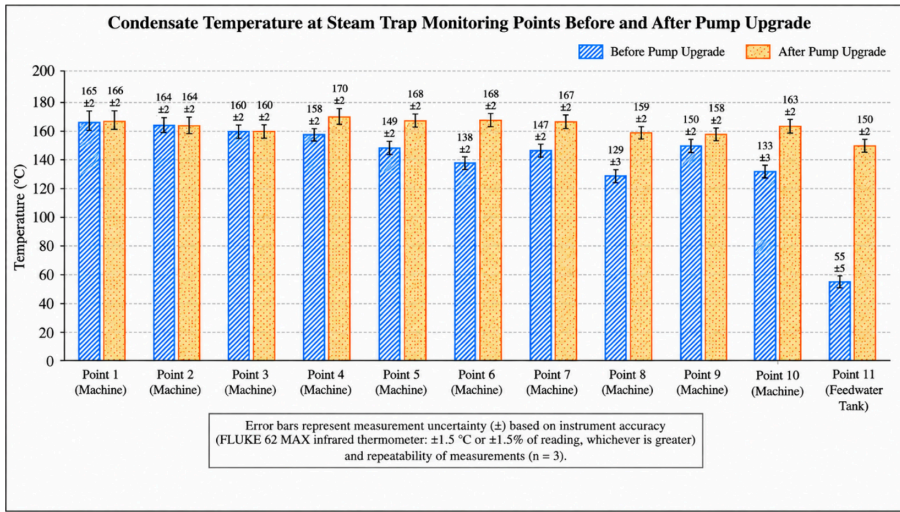
Fig. 2. Measured surface temperatures at 11 condensate monitoring points before and after the pump-system upgrade. Error bars indicate measurement uncertainty.
