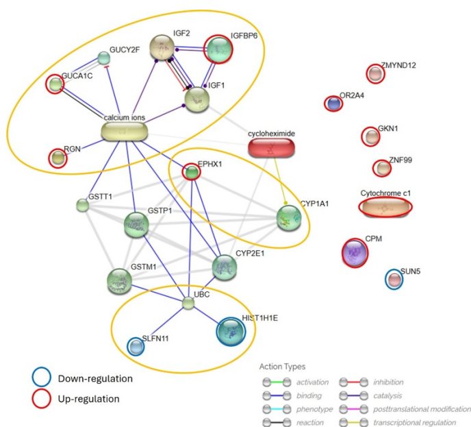
Fig. 4. Chemical-protein interaction network mapping CHX functional targets. The network details functional clusters in CHX-exposed HepG2 cells, comprising xenobiotic metabolism, the ubiquitin proteasome (UPS) and calcium signaling pathways, which are highlighted by yellow ellipses. Network construction using the STITCH 5.0 database (accessed in June 2026) indicates interactions between CHX and six candidate proteins, including the down-regulated SLFN11 and HIST1H1E and the up-regulated RGN, GUCA1C, and IGFBP6. Seven other proteins are shown as non-interacting. Abbreviations: SLFN11, Schlafen family member 11; HIST1H1E, histone cluster 1; RGN, regucalcin; GUCA1C, guanylate cyclase activator 1C; IGFBP6, insulin-like growth factor binding protein 6; EPHX1, epoxide hydrolase 1.
