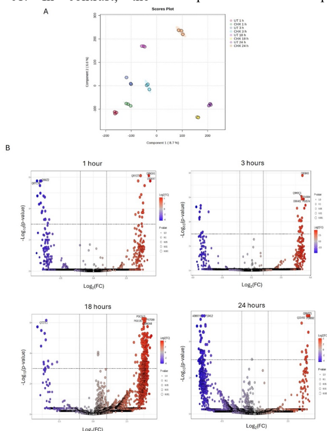
Fig. 3. DEPs identified by LC-MS/MS. (A) PLS-DA of 19,482 DEPs distinguishing between untreated and CHX-treated proteomes at 1, 3, 18 and 24 hours. (FDR < 0.05) (B) Volcano plots of all quantified proteins at each time point (X-axis: \log_2 fold change; Y-axis: -\log_{10} FDR-adjusted P -value). Blue and red dots indicate significantly downregulated ( \log_2 FC < -4.0 , P < 0.001 ) and upregulated ( \log_2 FC > 4.0 , P < 0.001 ) proteins in the CHX-treated proteome, respectively. The top five DEPs in each time point are labeled. Abbreviations: GeLC-MS/MS, Gel-enhanced liquid chromatography-tandem mass spectrometry; FDR, False discovery rate; FC, Fold change.
