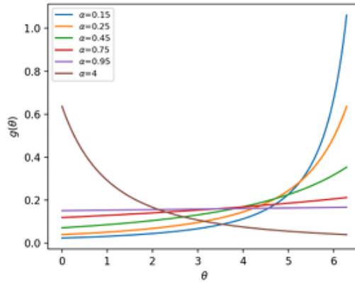
Fig. 1. MOECU density for several values of the parameter \alpha ; the density increases in \theta for \alpha < 1 and decreases in \theta for \alpha > 1 .
