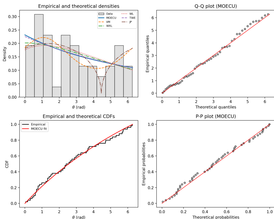
Fig. 3. Fitted densities (MOECU, VM, WXL, WL, TWE, JP) against the histogram of the FisherB4 data, and Q-Q, empirical/theoretical cdf, and P-P diagnostic plots for the MOECU fit.
