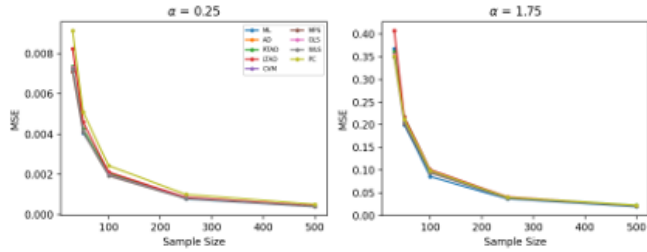
Fig. 2. Sample size n versus MSE.
