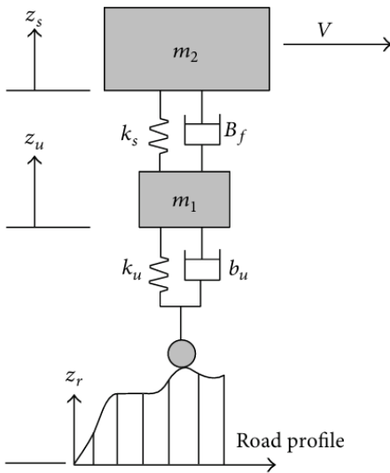
Fig. 5. Quarter truck suspension model on road profile of nonlinear [51].
