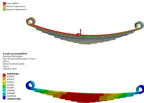
Fig. 6. Finite element model of the leaf spring.
