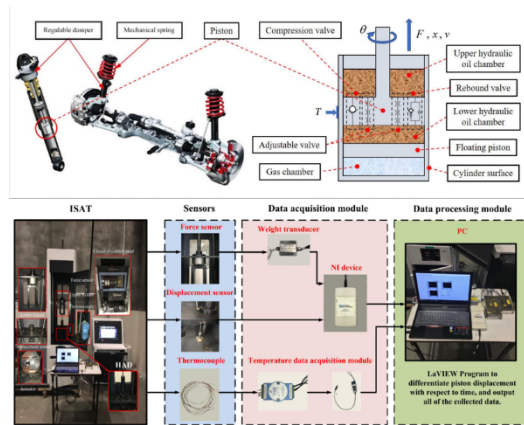
Fig. 8. Adaptive Artificial Neural Network Surrogate Model of Nonlinear Hydraulic Adjustable Damper, Commercial Semi-Active suspension stem and Schematic diagram of the damper (SAS system with the nonlinear HAD), Ther process of data collection [97].
