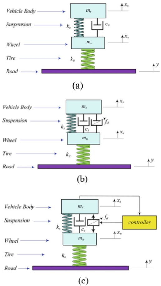
Fig. 2. Schematic diagrams of several types of vehicle suspension system [27] (a) Passive suspension system; (b) A semi-active suspension model; (c) A semi-active suspension model.
