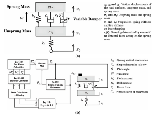
Fig. 10. The proposed enhanced energy-efficient skyhook control [33]: (a) quarter-car model of a semi-active suspension system; (b) block diagram of the control system. Semi-active suspension system.
