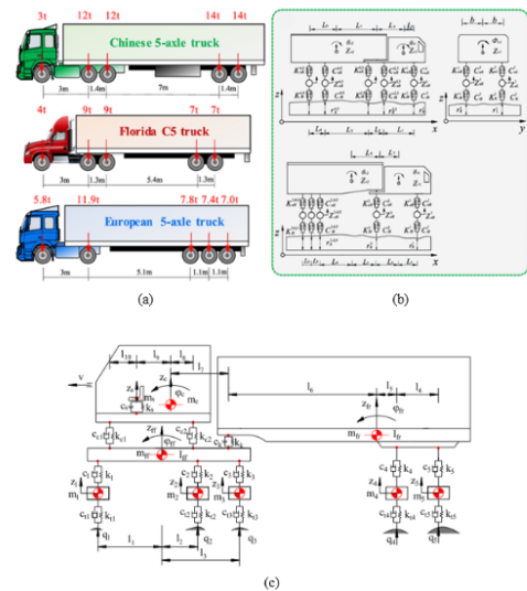
Fig. 3. Configurations of three typical trucks, truck semi-trailer (a) axle weight and spacings (b) analytical truck model (refined tire model unassembled) (c) articulated truck semi-trailer dynamic model [43, 66].
