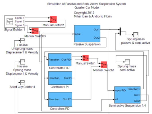
Fig. 7. The MATLAB suspension simulation scheme, quarter car model development of Computational and Mathematical Nonlinear Vibration Models (50).
