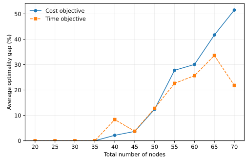
Fig. 4. Average optimality gaps for the single-objective models.
