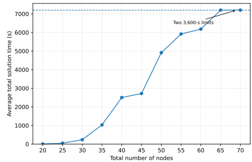
Fig. 3. Average total solution time for the two single-objective models.
