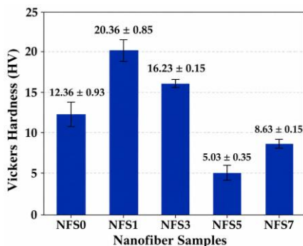
Fig. 7. Average Vickers hardness of PVA/Silica nanofibers.
