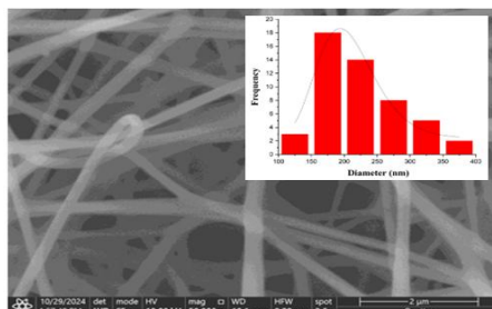
Fig. 3. FESEM image, and diameter distribution of sample NFS1.
