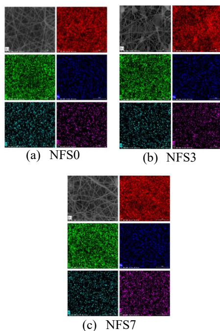
Fig. 9. FESEM images and corresponding EDS elemental maps of (a) NFS0, (b) NFS3, and (c) NFS7 PVA/silica nanofiber membranes.
