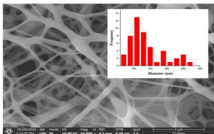
Fig. 5. FESEM image, and diameter distribution of sample NFS5.
