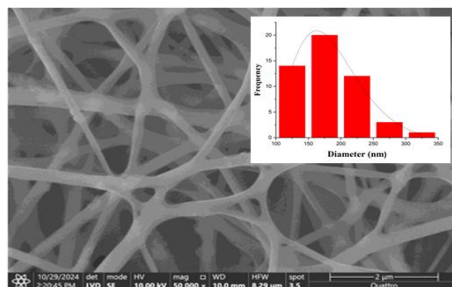
Fig. 6. FESEM image, and diameter distribution of sample NFS7.
