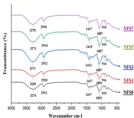
Fig. 11. FTIR spectra of PVA/silica nanofibers with different silica loadings (NFS0–NFS7).
