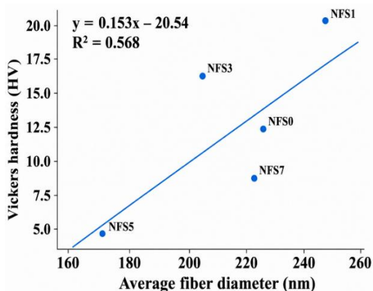
Fig. 8. Relationship between average fiber diameter and Vickers hardness of PVA/silica nanofiber membranes with different silica contents.
