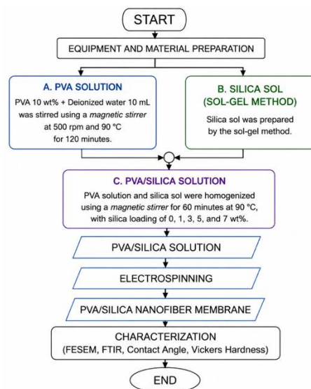
Fig. 1. Schematic representation of the fabrication process of geothermal silica-based PVA nanofiber membranes via electrospinning.
