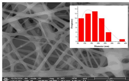
Fig. 4. FESEM image, and diameter distribution of sample NFS3.
