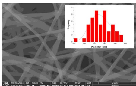
Fig. 2. FESEM image, and diameter distribution of sample NFS0.
