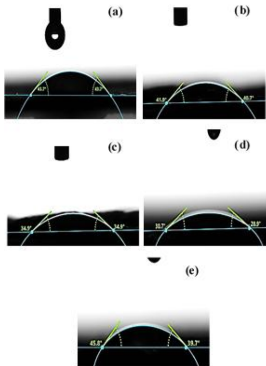
Fig. 10. Contact angle measurements of nanofiber membranes: (a) NFS0, (b) NFS1, (c) NFS3, (d) NFS5, and (e) NFS7, using water droplets at 20 °C.
