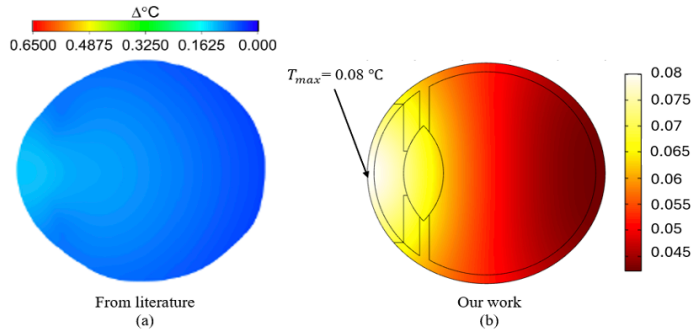
Fig. 5. Temperature distribution in the eye for 700 MHz frequency at 0.35 mW power (a) literature, and (b) present work.
