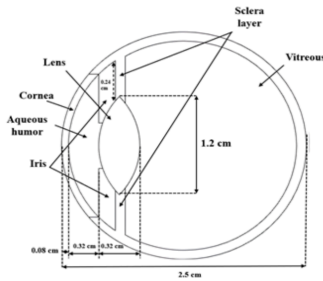
Fig. 3. Heterogenous model of human eye.
