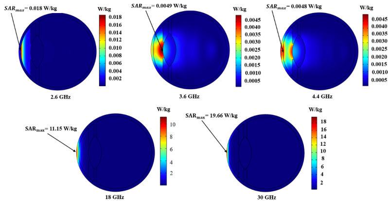
Fig. 8. Specific Absorption Rate (SAR) in the eye at different 5G frequencies at 0.1W radiated power
