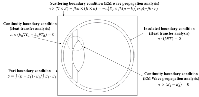
Fig. 4. Boundary conditions for Electromagnetic wave and Bioheat Transfer.
