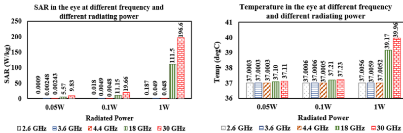
Fig. 10. (a) SAR in the eye at different radiated powers, and (b) temperature in the eye at different radiated powers for 30 min exposure.
