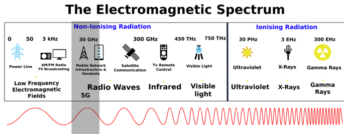
Fig. 1. Electromagnetic spectrum.
