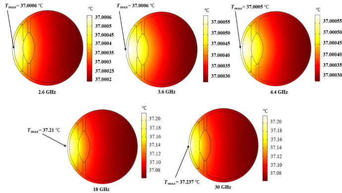
Fig. 9. Temperature distribution in the eye at different 5g frequencies at 0.1 W radiated power for 30 minutes.
