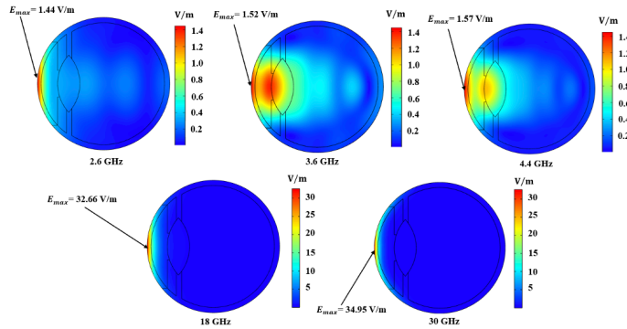
Fig. 7. Electric field distribution in the eye at different 5G frequencies at 0.1 W radiated power.
