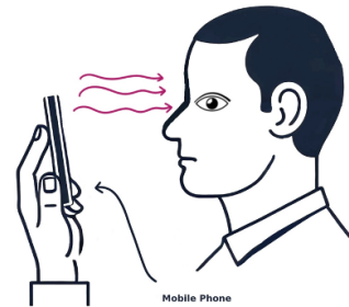
Fig. 2. Human eyes getting exposed to the 5G radiation from a cell phone.
