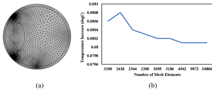
Fig. 6. (a) 2D mesh model of human eye, and (b) mesh convergence graph between temperature and mesh elements.
