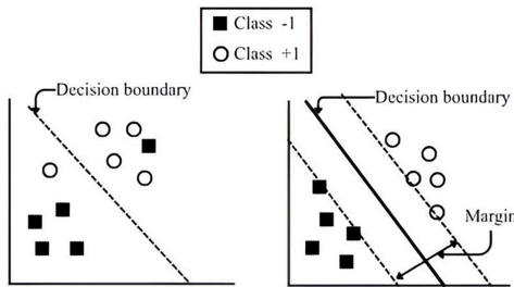
Fig. 2. Illustration of the SVM Concept. Adapted from [31].
