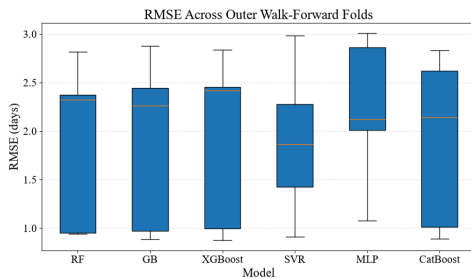
Fig. 2. RMSE distributions across the five outer walk-forward validation folds.
