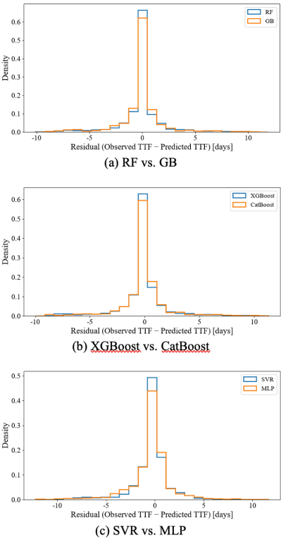
Fig. 4. Residual distributions of TTF prediction models.
