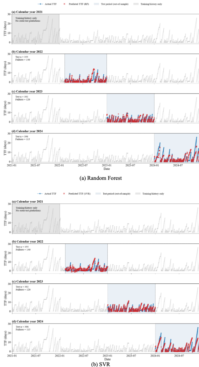
Fig. 3. True vs. predicted TTF for Random Forest and SVR: nested cross-validation results.
