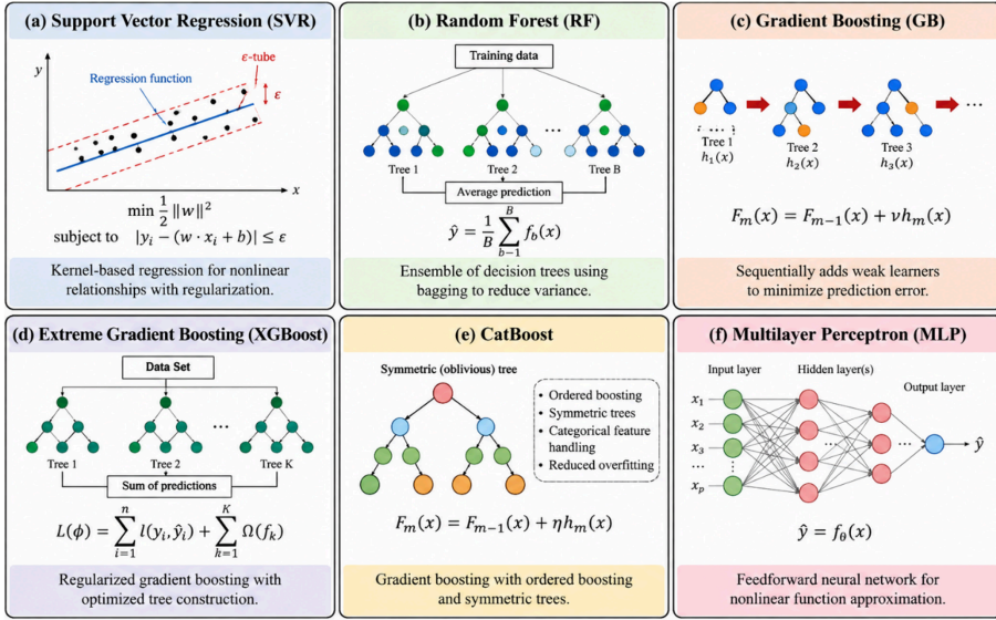
Fig. 1. Structural and mechanical differences in TTF prediction modeling paradigms.
