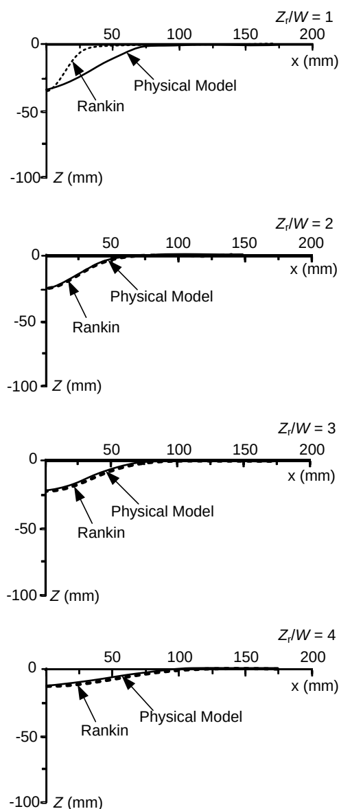
Fig.7. Surface settlement troughs for different values of Z_r/W , where H = 50 mm and L = 250 mm.
