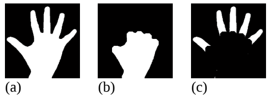
Fig.2. Raw results of the top-hat transform (a) hand (b) hand blob and (c) fingers.
