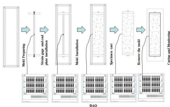
Fig.6. Step of internal restrained expansion test.
