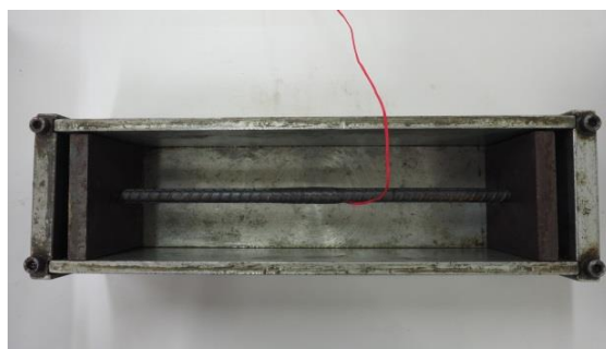
7(a) before casting
