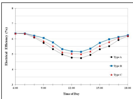
Fig.5. Hourly Variations of Simulated Electrical Efficiency.
