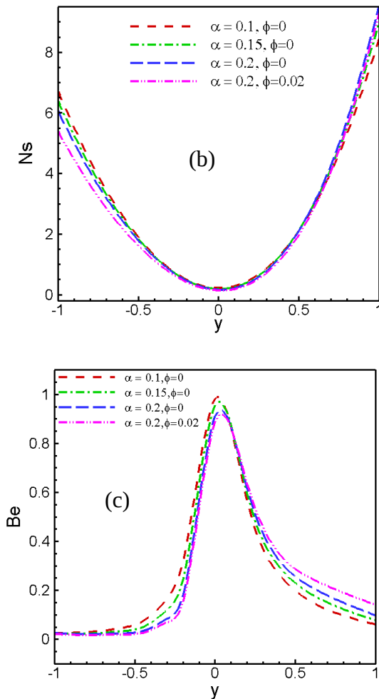
Fig.5. Effect of thermal conductivity variation parameter on (a) temperature profile, (b) entropy generation rate and (c) Bejan profiles respectively at Pr=7.1, Gr=1, Br=7.1, N=1, Re=1, Ha=1, R=1 .
