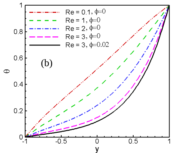
Fig.3. Effect of Reynolds number on (a) velocity profiles and (b) temperature distributions respectively
