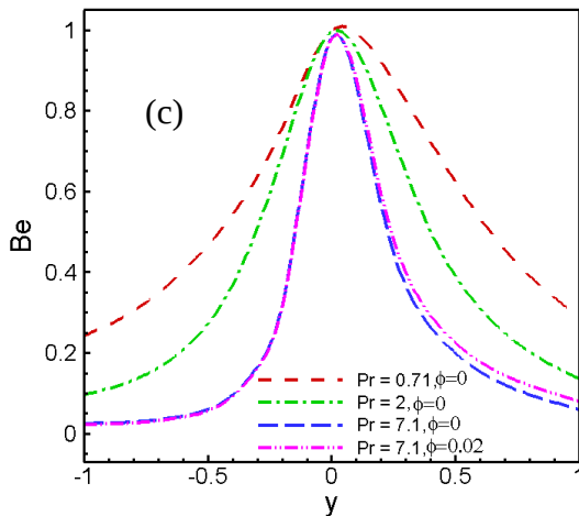
Fig.7. Effect of Prandtl number on (a) temperature profile, (b) entropy generation rate and (c) Bejan profiles respectively at R=1, Gr=1, Br=7.1, N=1, Re=1, Ha=1, \alpha=0.1 .
