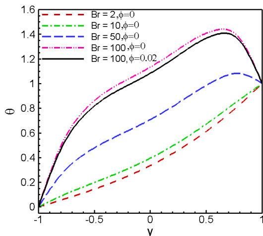
Fig. 10. Effect of Brinkman number on temperature profile at R=1, Gr=1, N=1, Pr=7.1, Re=1, Ha=1, \alpha=0.1 .
