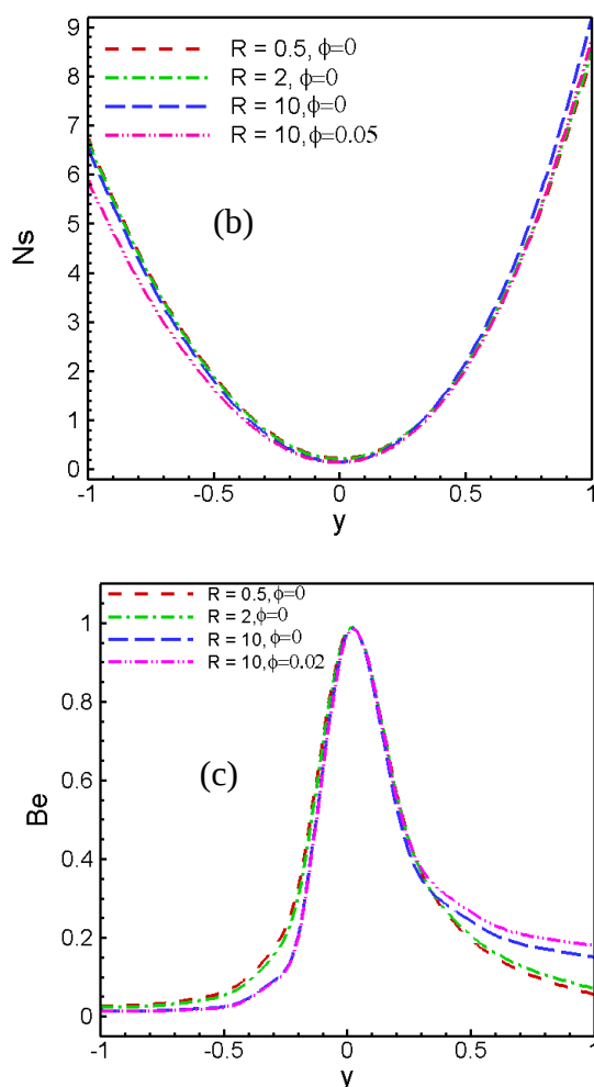
Fig.6. Effect of Radiation parameter on (a) temperature profile, (b) entropy generation rate and (c) Bejan profiles respectively at Pr=7.1, Gr=1, Br=7.1, N=1, Re=1, Ha=1, \alpha=0.1 .
