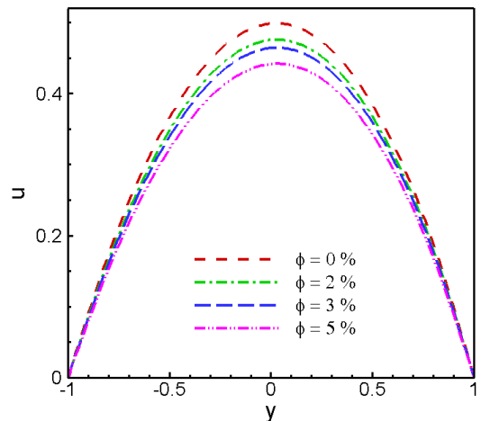
Fig.9. Effect of nanoparticles volume fraction on velocity profiles at Br=7.1, Gr=1, \alpha=0.1, Re=1, R=1, Pr=7.1, Ha=1 .
