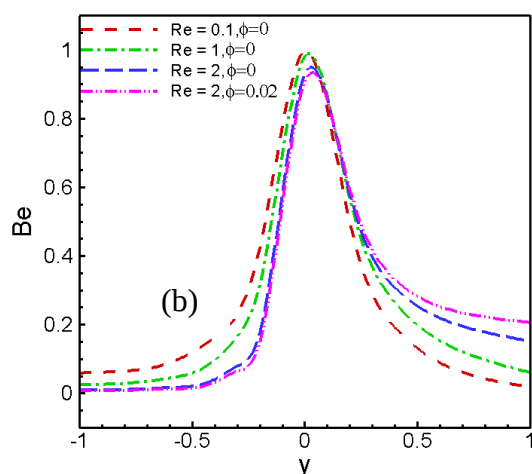
Fig.4. Effect of Reynolds number on (a) entropy generation rate and (b) Bejan profiles respectively at
