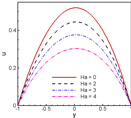
Fig.8. Effect of Hartmann number on velocity profile at Br=7.1, Gr=1, \alpha=0.1, Re=1, R=1, Pr=7.1, \phi=0
