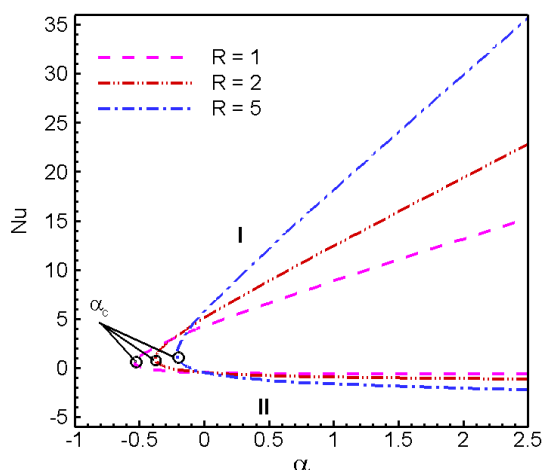
Fig.2. Approximate bifurcation diagrams of \alpha in the (\alpha, Nu(1)) plane for different values of R obtained by Drazin-Tourigny method (1996)
