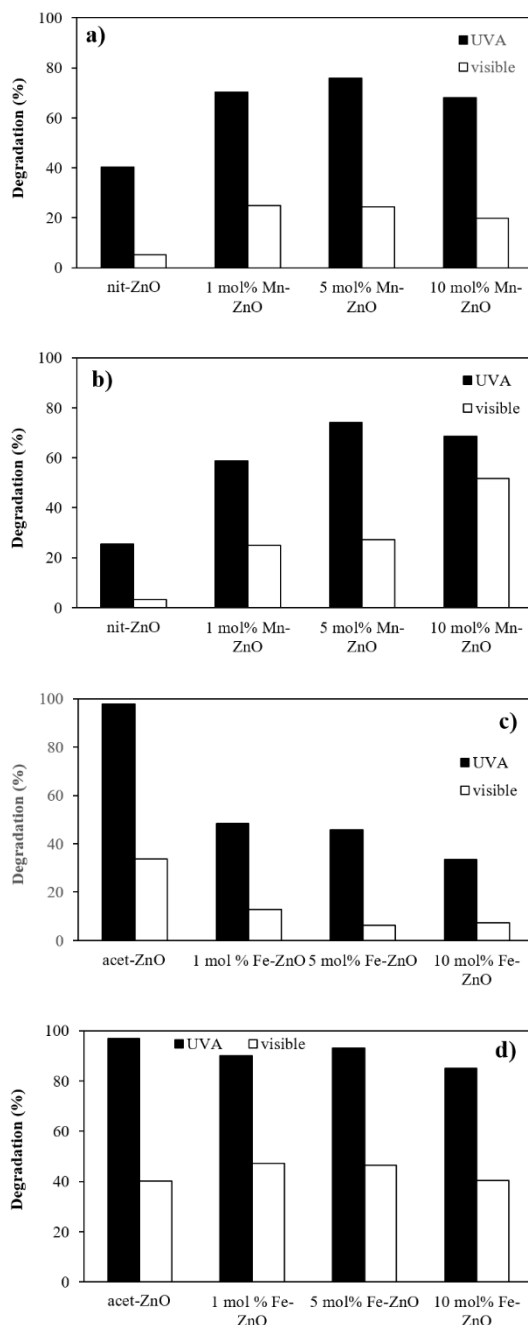
Figure 3. Degradation MB (a, c) and AM (b, d) by pristine and doped ZnO under visible and UVA light (catalyst concentration = 1 g/L, dye concentration = 10 mg/L, pH = 7, and irradiation time 90 min).
