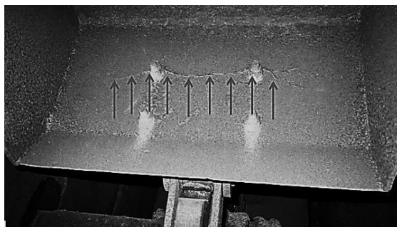
Figure 2 The main crack between two holes with branch cracks present at both edges.
