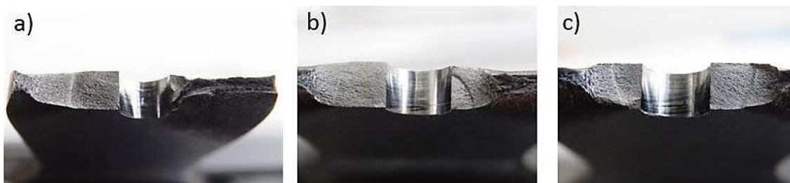
Figure 10 Fracture surface of a) SD, b) SNC and c) ENC fatigue specimen tested at stress amplitude of 96 MPa.
