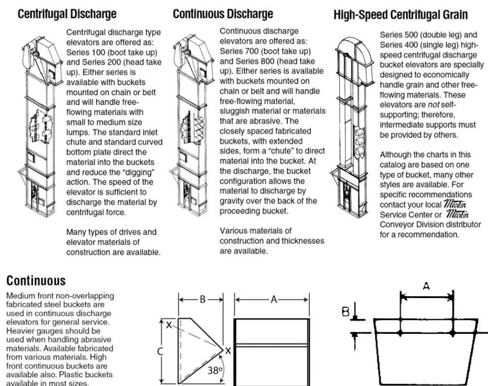
Figure 1 Various types of bucket elevators used in industry [1]
