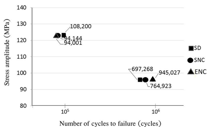
Figure 8 S-N graph of fatigue specimen which has hole at the center of the specimen
