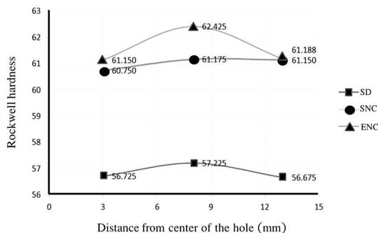
Figure 7 Average Rockwell hardness value at various distances from the center of the hole
