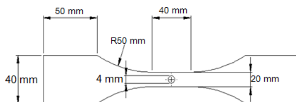
Figure 3 Shape and dimensions of fatigue test specimen with a 4-mm diameter hole
