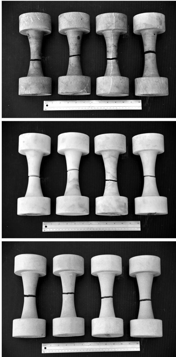
Figure 4 Post-test specimens of SB limestone (top), SB marble (middle) and PP sandstone (bottom).
