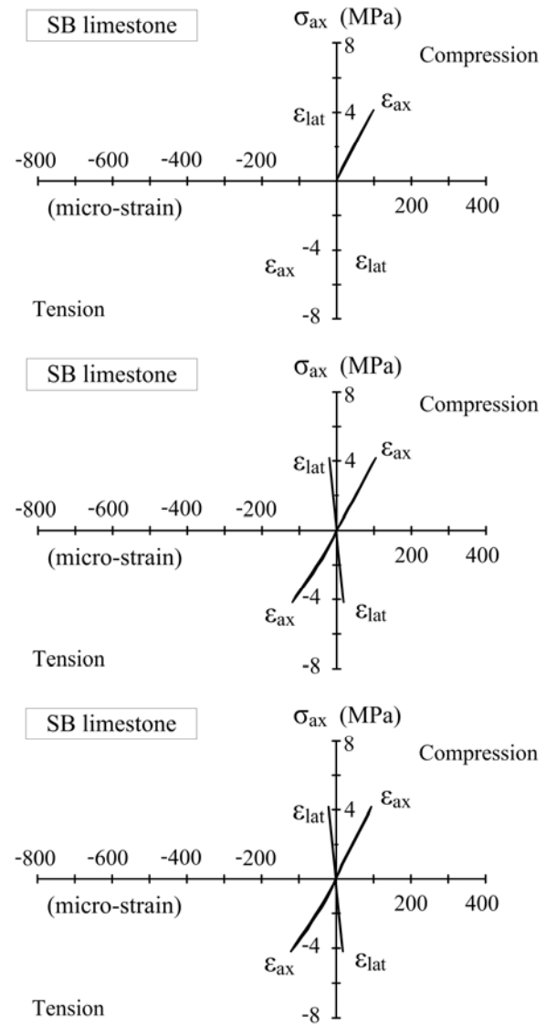
Figure 7 Axial stress ( \sigma_{ax} ) as a function of axial and lateral strains ( \epsilon_{ax} , \epsilon_{lat} ) for one cycle of compression and tension loading of SB limestone specimens.
