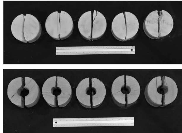
Figure 5 Some post-test specimens from Brazilian (top) and ring (bottom) tensile strength testing.
