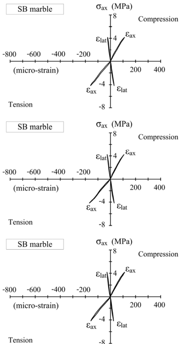
Figure 8 Axial stress ( \sigma_{ax} ) as a function of axial and lateral strains ( \epsilon_{ax} , \epsilon_{lat} ) for one cycle of compression and tension loading of SB marble specimens.
