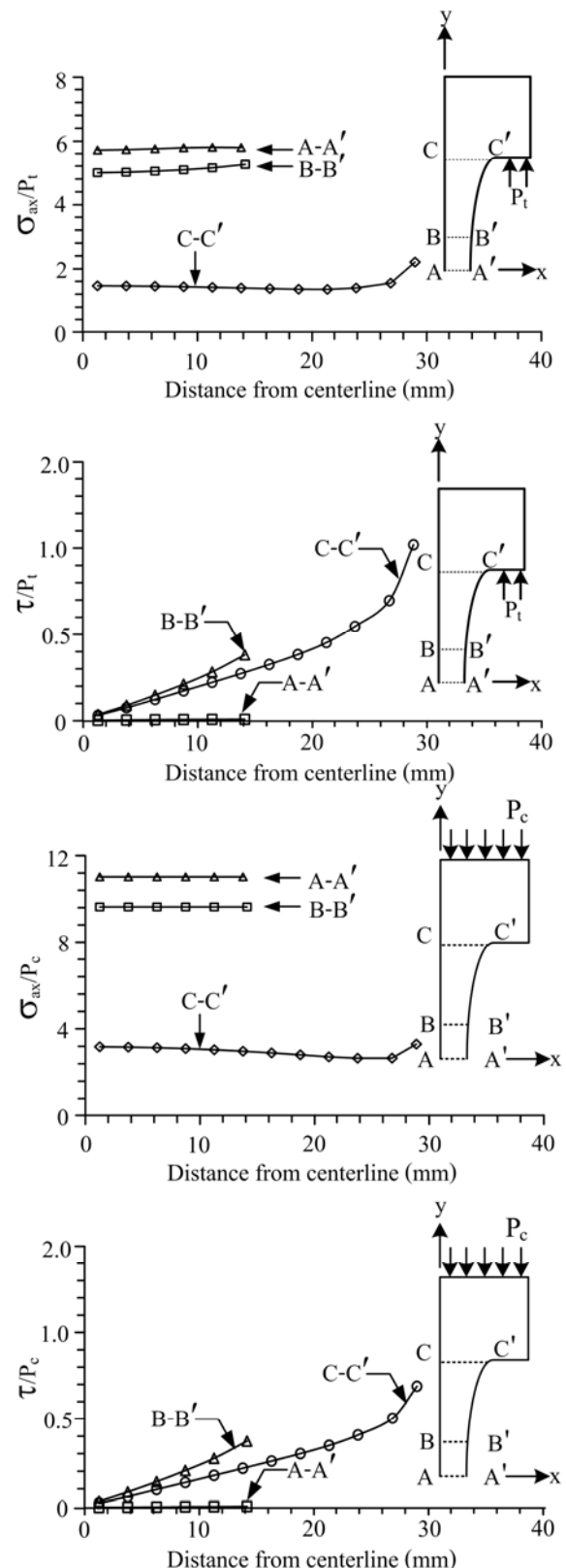
Figure 3 Axial and shear stresses across specimen diameters for tensile loading (top two) and compressive loading (bottom two).
