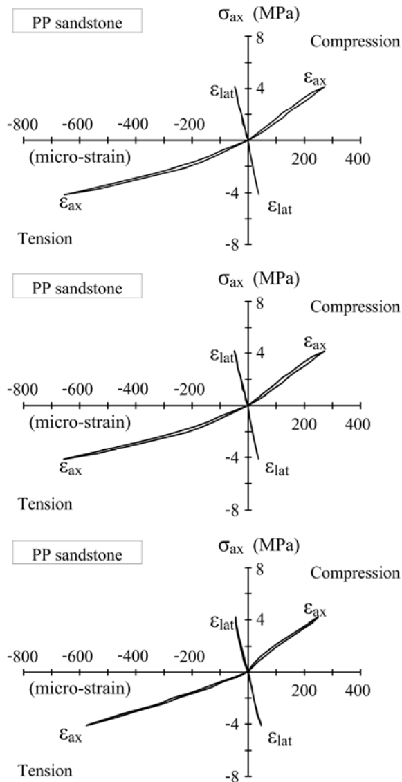
Figure 6 Axial stress ( \sigma_{ax} ) as a function of axial and lateral strains ( \epsilon_{ax} , \epsilon_{lat} ) for one cycle of compression and tension loading of PP sandstone specimens.
