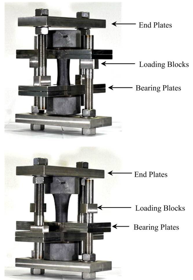
Figure 1 Compression-to-tension load converter arranged for tensile loading (top) and compressive loading (bottom).
