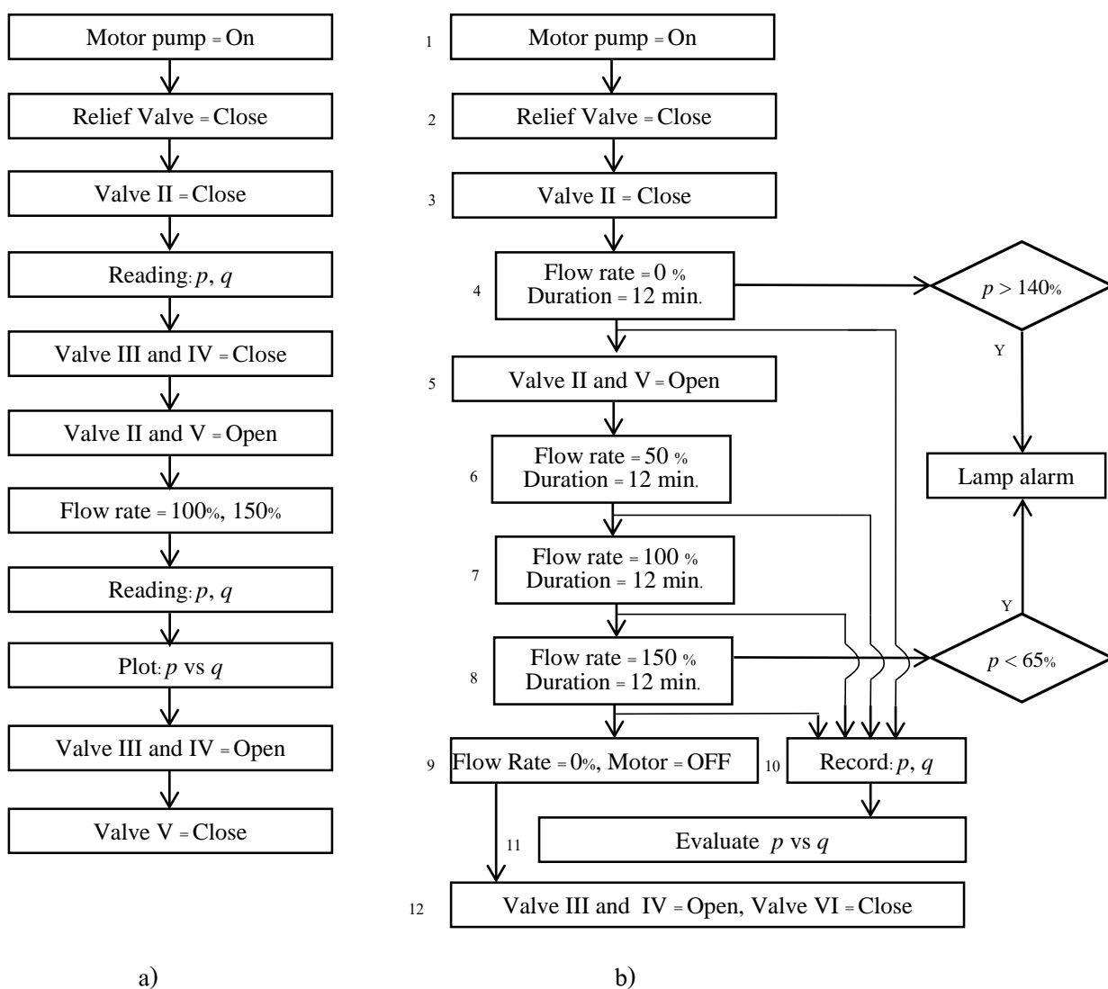
Figure 5 a) Flow Diagram of fire pump performance testing procedure, and b) Block diagram for the automated testing system.
