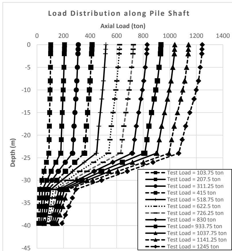
Figure 8. Load distribution along 1.2 m-diameter pile shaft analyzed by PLAXIS 3D.
