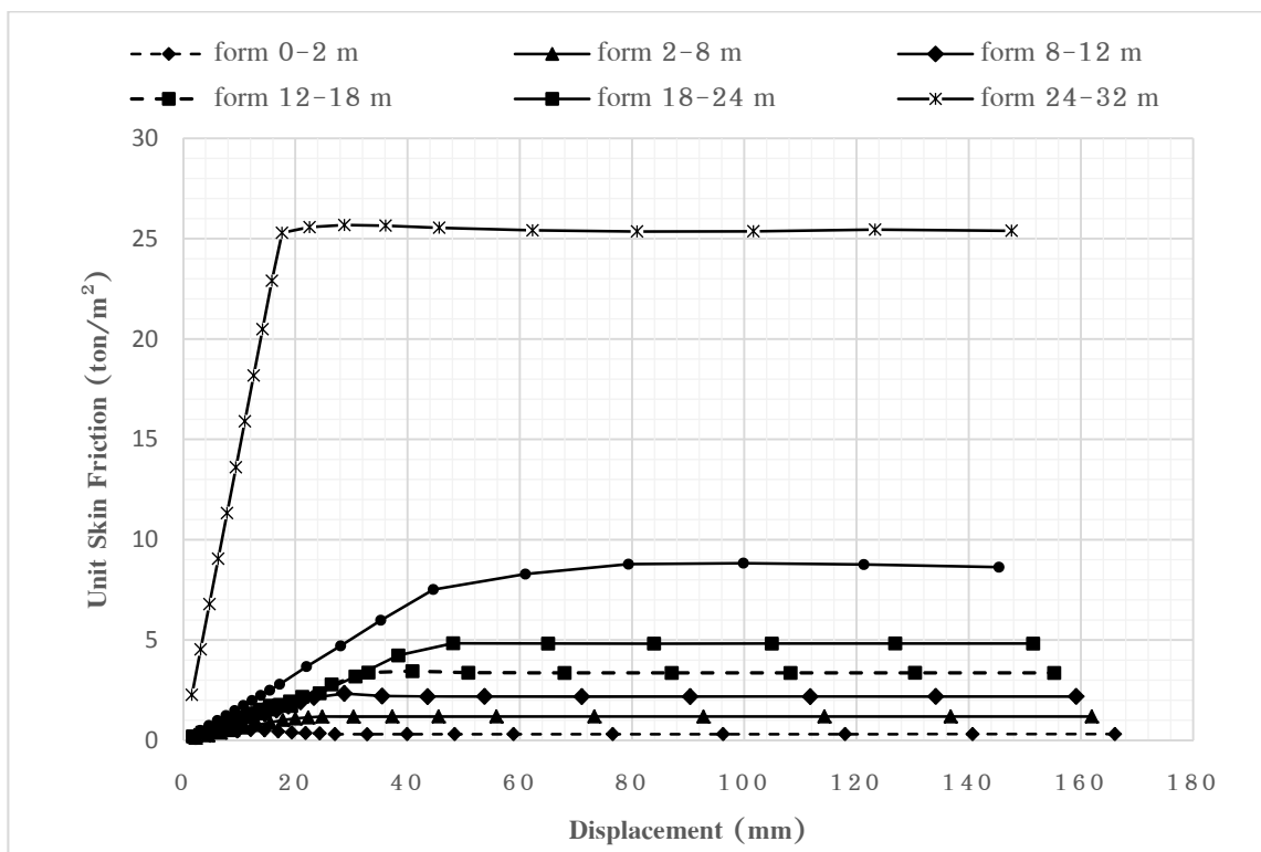
Figure 10. Mobilized skin friction of 1.2 m- \phi pile shaft analyzed by PLAXIS 3D with 5 times of design load.
