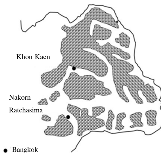
Figure 2. Distribution of loess in Northeastern Thailand. [2]
