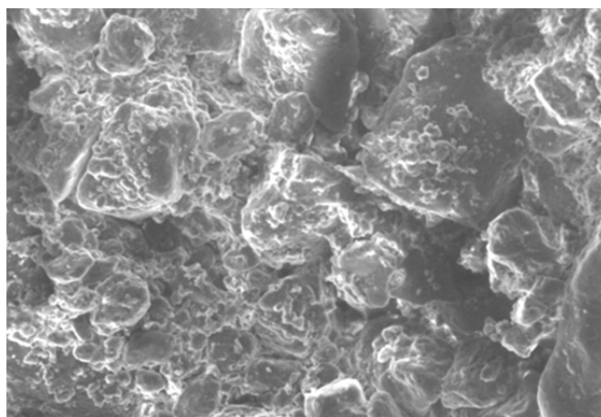
Figure 3. Khon Kaen loess. [1]
