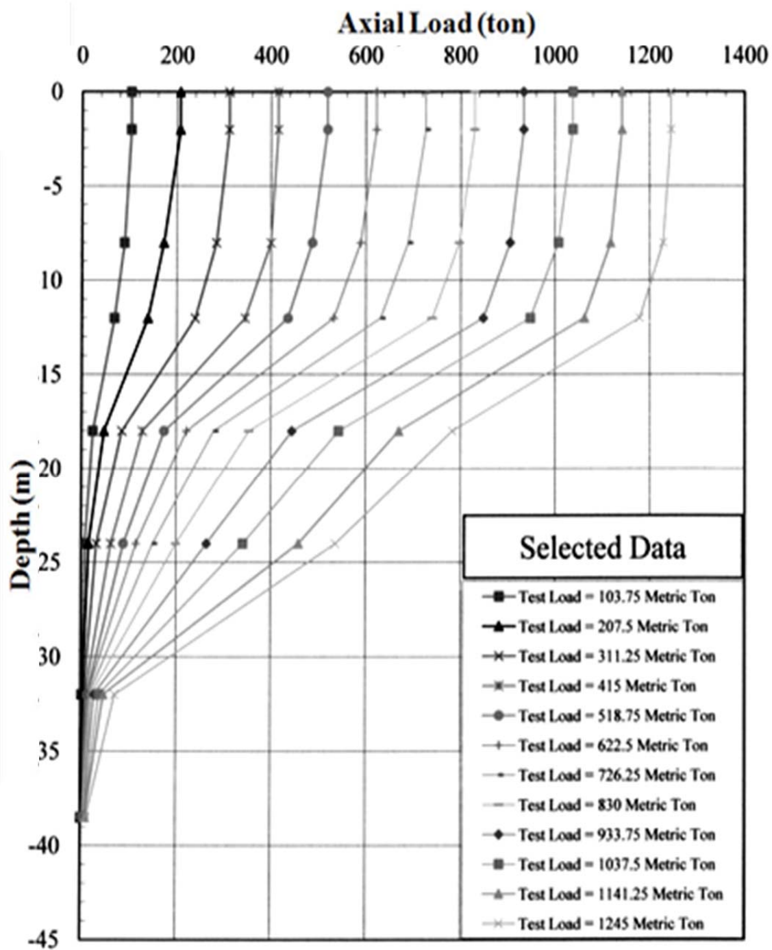
Figure 7. Load distribution along 1.2 m-diameter pile shaft.
