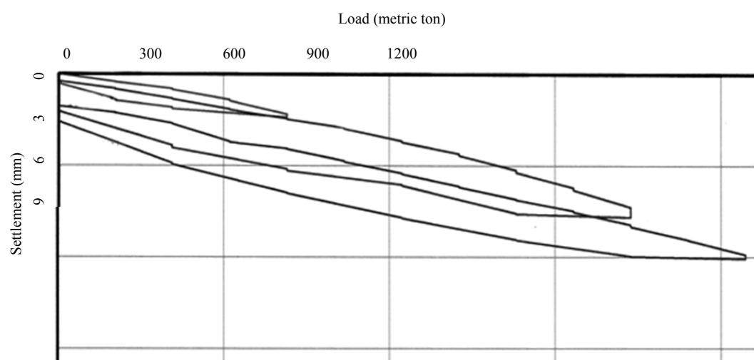
Figure 6. Static pile load test result of 1.2 m–diameter pile.
