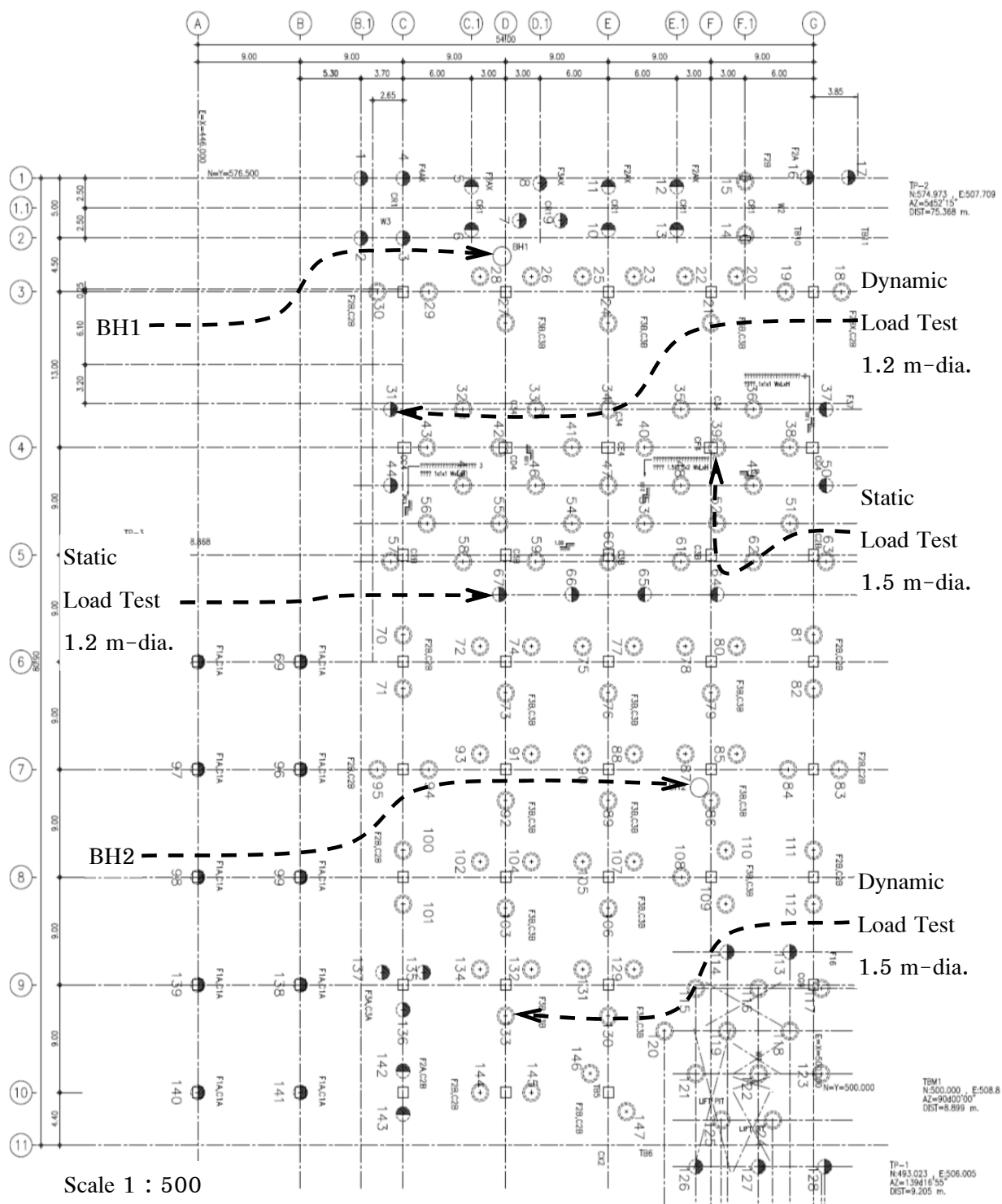
Figure 4. Site plan.
