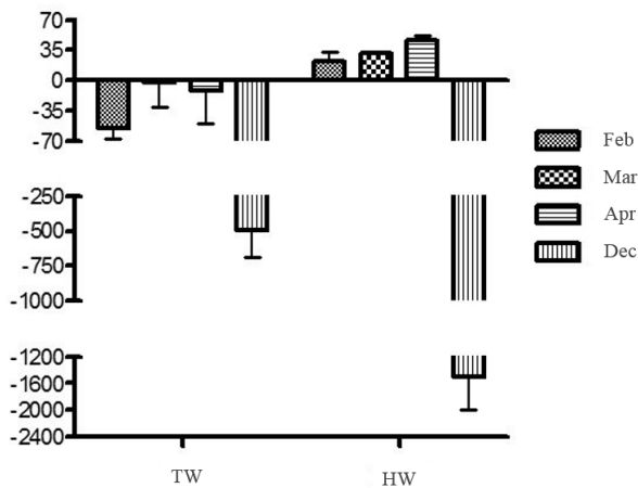
Figure 4. Flux of SRP ( \mu\text{mol}/\text{m}^2/\text{day} ) in sediment cores incubated under oxic environment.
