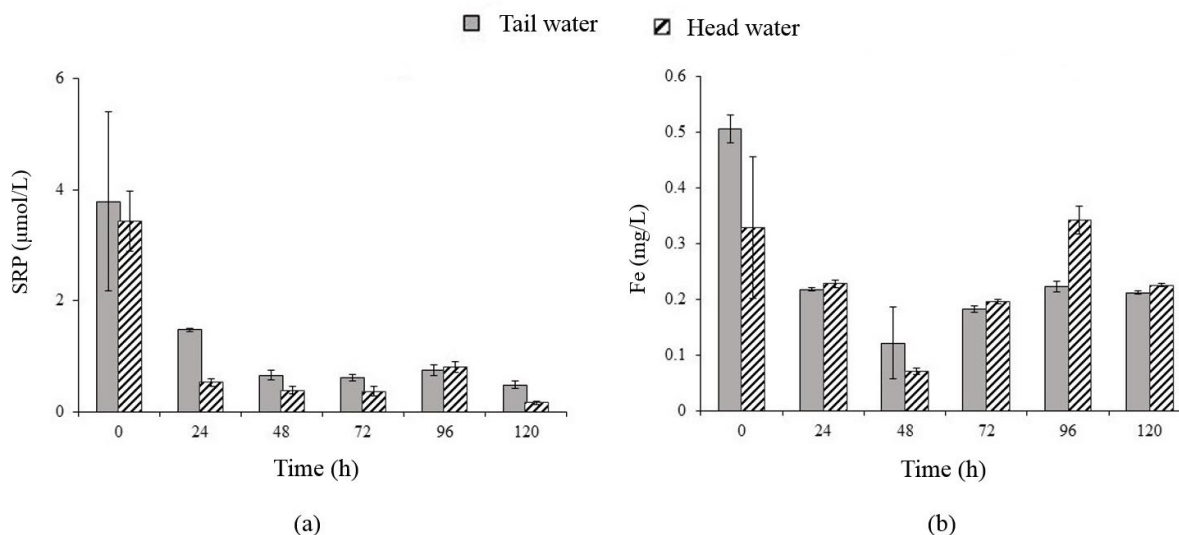
Figure 6. (a) Flux of SRP in sediment cores incubated under continuous aeration and (b) depletion of Fe from the overlying water in sediment cores.
