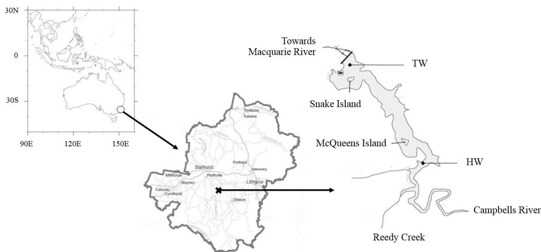
Figure 1. Location of Ben Chifley reservoir and two sampling sites, tail water (TW) and head water (HW).
