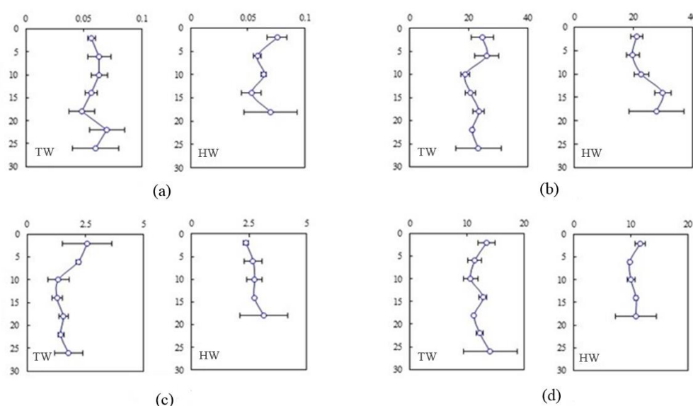
Figure 3. Depth distribution of P fraction ( \mu\text{g}/\text{g} ) in sediment cores collected from tail water (TW) and head water (HW). (a) Loosely bound P, (b) Fe and Al - bound P, (c) Ca - bound P and (d) residual P.
