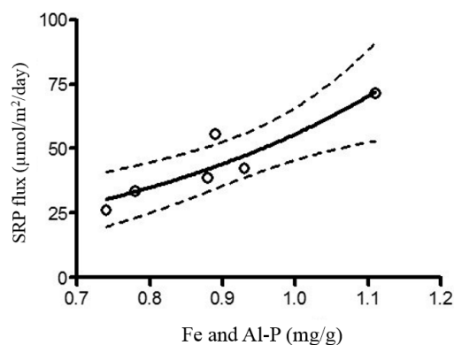
Figure 7. Correlation between SRP flux and the concentration of Fe and Al-P in the sediment core incubated under aerated environment (dashed line represents 95% C.I.).
