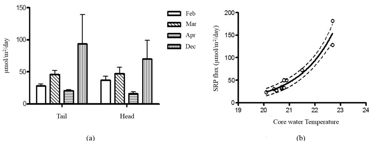
Figure 5. (a) Flux of SRP in sediment cores incubated under anoxic environment and (b) relationship between SRP flux and the temperature of overlying water in sediment core (dashed line represents 95% C.I).
