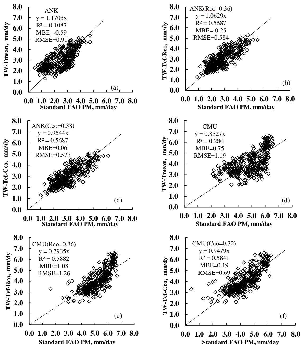
Figure 2. Regression between the daily ETo estimated by the standard FAO PM method and the Thornthwaite method (TW) with mean temperature (Tmean), effective temperature (Tef), recommended coefficient (Rco), and locally calibrated coefficient (Cco) for ANK ((a), (b) and (c)) and CMU ((d), (e) and (f)), and also the mean bias error (MBE) and the root mean square error (RMSE) from the comparison between them
