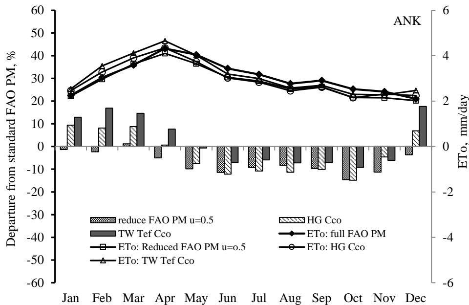
Figure 3. Comparison of the ETo values (line) and the percentage departure values from the standard ETo (bar) between the method of reduced FAO PM u=0.5 , the Hargreaves method with calibrated coefficient (HG Cco), and the Thornthwaite method with effective temperature and calibration coefficient (TW TefCco) in the Angkhang (ANK) station
