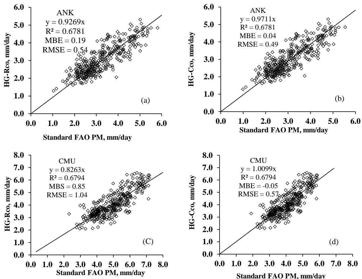
Figure 1. Regression between the daily ETo estimated by the standard FAO PM method and the Hargreaves method (HG) with recommended coefficient (Rco) and locally calibrated coefficient (Cco) for ANK ((a) and (b)) and CMU ((c) and (d)), and also the mean bias error (MBE) and the root mean square error (RMSE) from the comparison between them
