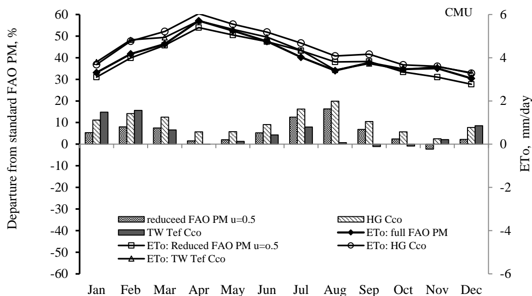
Figure 4. Comparison of the ETo values (line) and the percentage departure values from the standard ETo (bar) between the method of reduced FAO PM u=0.5 , the Hargreaves method with calibrated coefficient (HG Cco), and the Thornthwaite method with effective temperature and calibration coefficient (TW TefCco) in the Chiang Mai University (CMU) station
