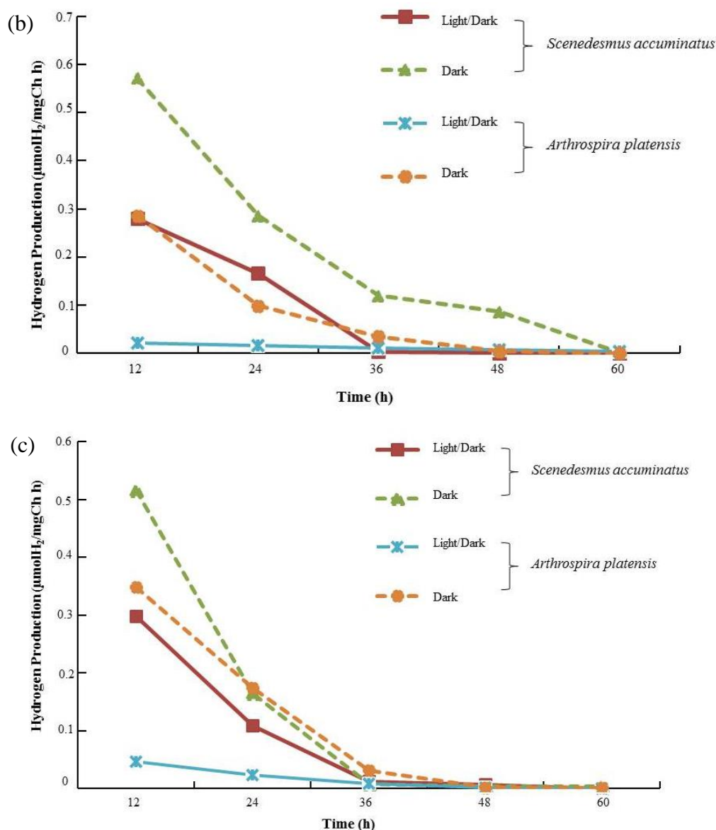
Figure 3. Effect of atmospheric gas conditions on H 2 production: (a) 100% argon; (b) 99% argon + 1% CO 2 ; and (c) 98% argon + 2% CO 2 (cont.)
