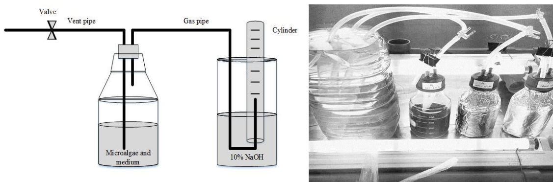
Figure 1. A schematic of the photoreactors for H 2 production from microalgae
