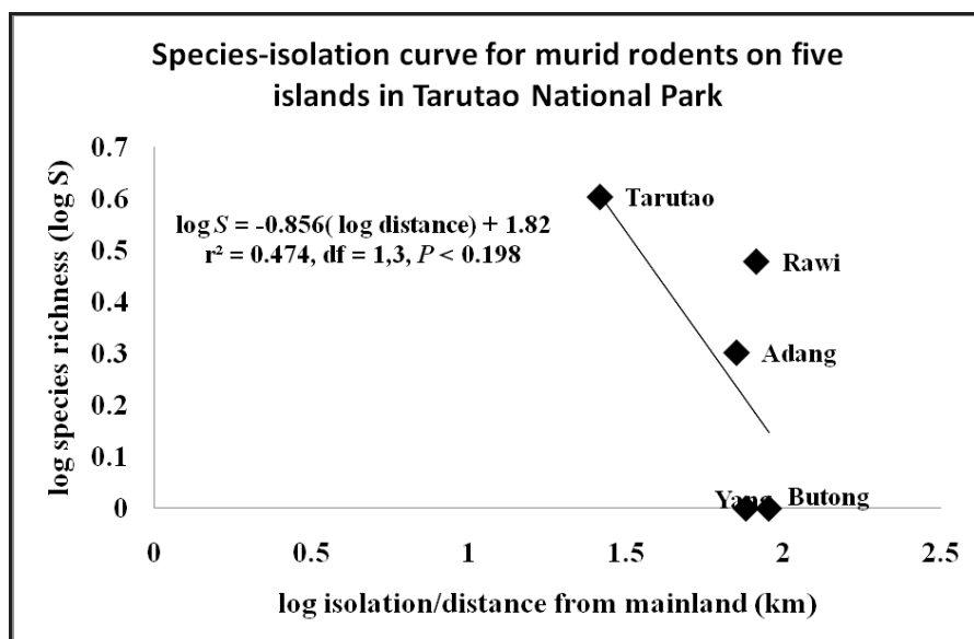
Figure 4 Species-isolation curve of murid rodents based on the individuals captured. The graph follows the Arrhenius equation, \log_{10} S = c + z \log_{10} D .
