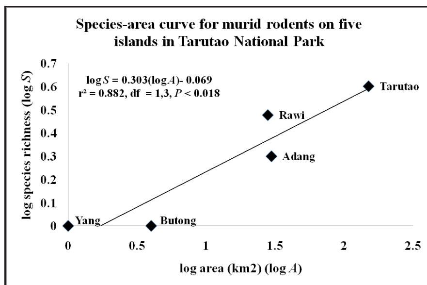
Figure 3 Species-area curve of murid rodents based on the individuals captured. The graph follows the Arrhenius equation, \log_{10} S = c + z \log_{10} A .
