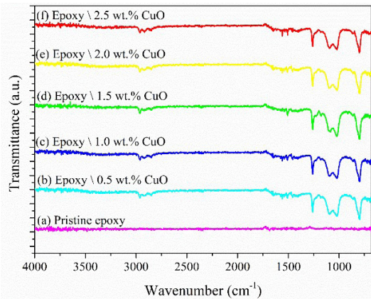
Figure 7: FTIR spectra of (a) Pristine epoxy and nano-CuO polymer composites with (b) 0.5 wt.%, (c) 1.0 wt.%, (d) 1.5 wt. %, (e) 2.0 wt. %, and (f) 2.5 wt.% of CuO nanoparticles loading.
