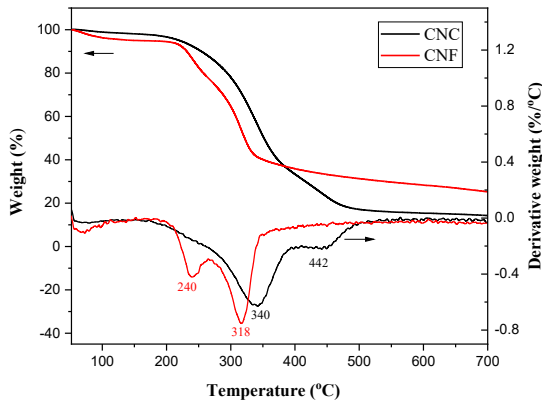
Figure 6: TGA curves of CNC and CNF samples synthesized by acid hydrolysis and by TEMPO oxidation, respectively.
