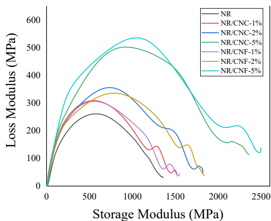
Figure 10: Cole-Cole plots of NR nanocomposites.
