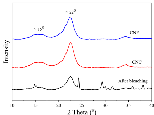
Figure 5: XRD patterns of samples following the bleaching process, hydrolyzed CNCs, and oxidized CNFs.
