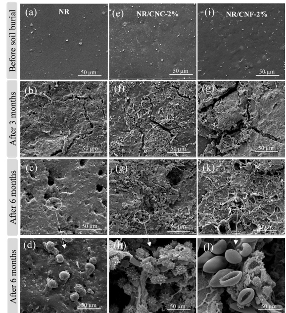
Figure 11: SEM analysis of NR nanocomposite films taken before and after soil burial for 3 and 6 months: (a)–(d) neat NR, (e)–(h) NR/CNC-2%, and (i)–(l) NR/CNF-2%.
