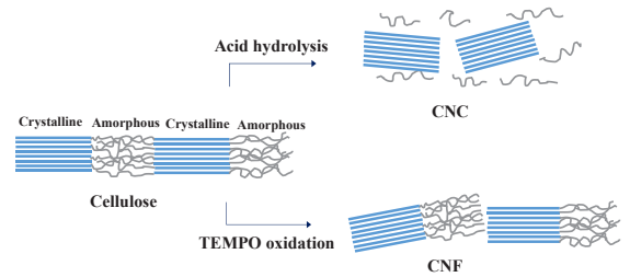
Figure 2: Schematic mechanisms of producing CNCs via acid hydrolysis and CNFs via TEMPO oxidation [23].
