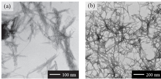
Figure 1: TEM images of (a) CNCs extracted by acid hydrolysis and (b) CNFs extracted by TEMPO oxidation.
