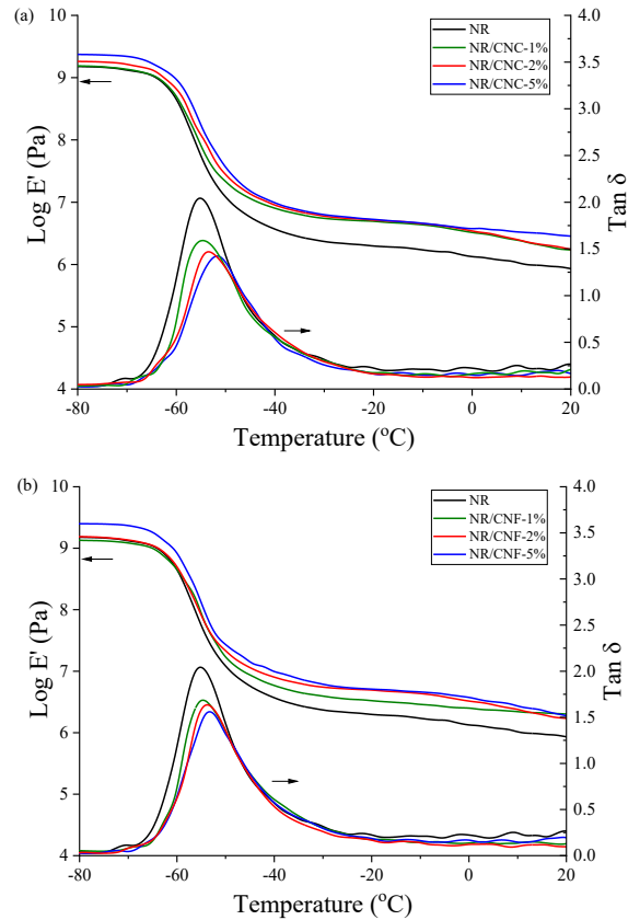
Figure 9: Storage modulus and \tan \delta from DMA analysis of (a) NR/CNC and (b) NR/CNF nanocomposite films.
