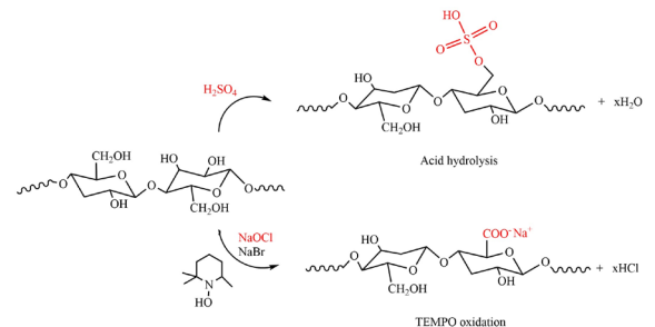
Figure 3: Chemical structures of CNCs and CNFs synthesized through acid hydrolysis and TEMPO oxidation, respectively [28].
