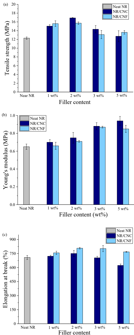
Figure 8: NR nanocomposite film mechanical properties: (a) tensile strength, (b) Young's modulus, and (c) elongation at break. At least five measurements were collected to calculate the mean and standard deviation.
