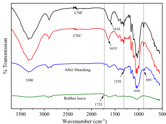
Figure 4: FTIR spectra of rubber leaf powders, bleached samples, hydrolyzed CNCs, and oxidized CNFs.
