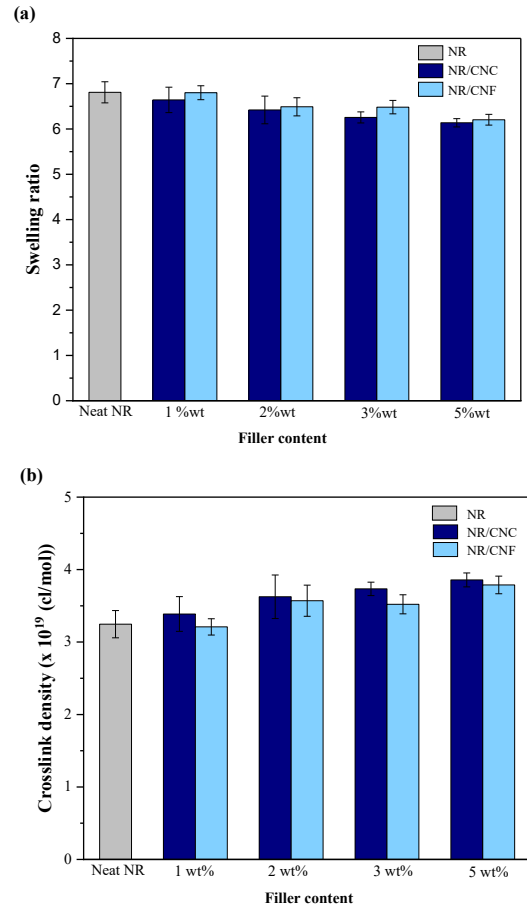
Figure 7: (a) Swelling ratio and (b) crosslink density of NR, NR/CNC, and NR/CNF nanocomposite films. At least five measurements were collected to calculate the mean and standard deviation.
