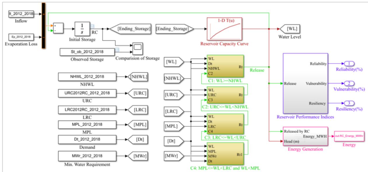
Fig. 2 The Water Balance-Based Reservoir Reoperation Model Using Adapted Rule Curve
