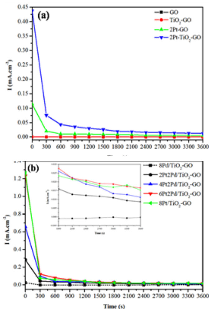
Figure 8 Chronoamperometric curves of GO, TiO 2 -GO, 2Pt-GO and 2Pt/TiO 2 -GO (a), xPt2Pd/TiO 2 -GO; x = 2, 4, 6 and 8 (b) in 0.5 M CH 3 OH and a 0.5 M H 2 SO 4 solution at specific potentials of these catalysts, 3600 s.
