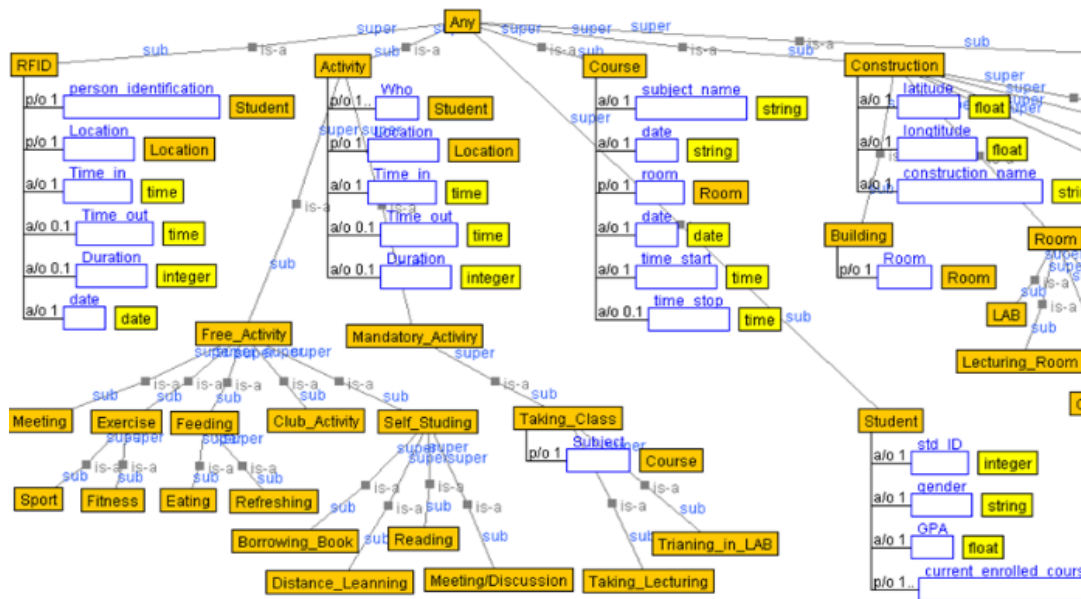
Figure 2 The ontology for activity in campus [19]
